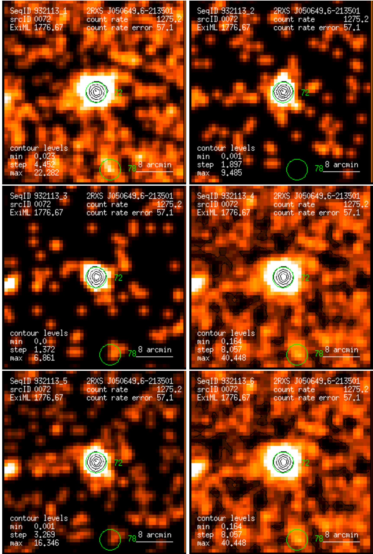
Figure 72: RASS 932113: detection 0072: band rate images, Gaussian filter: (1) PSPC channels 11 – 41, (2) 52 – 90, (3) 91 – 201, (4) 11 – 235, (5) 52 – 201, (6) 11 – 201. Broad band rates in counts/ks. Band rate contour levels in counts/ks/arcmin 2 .
