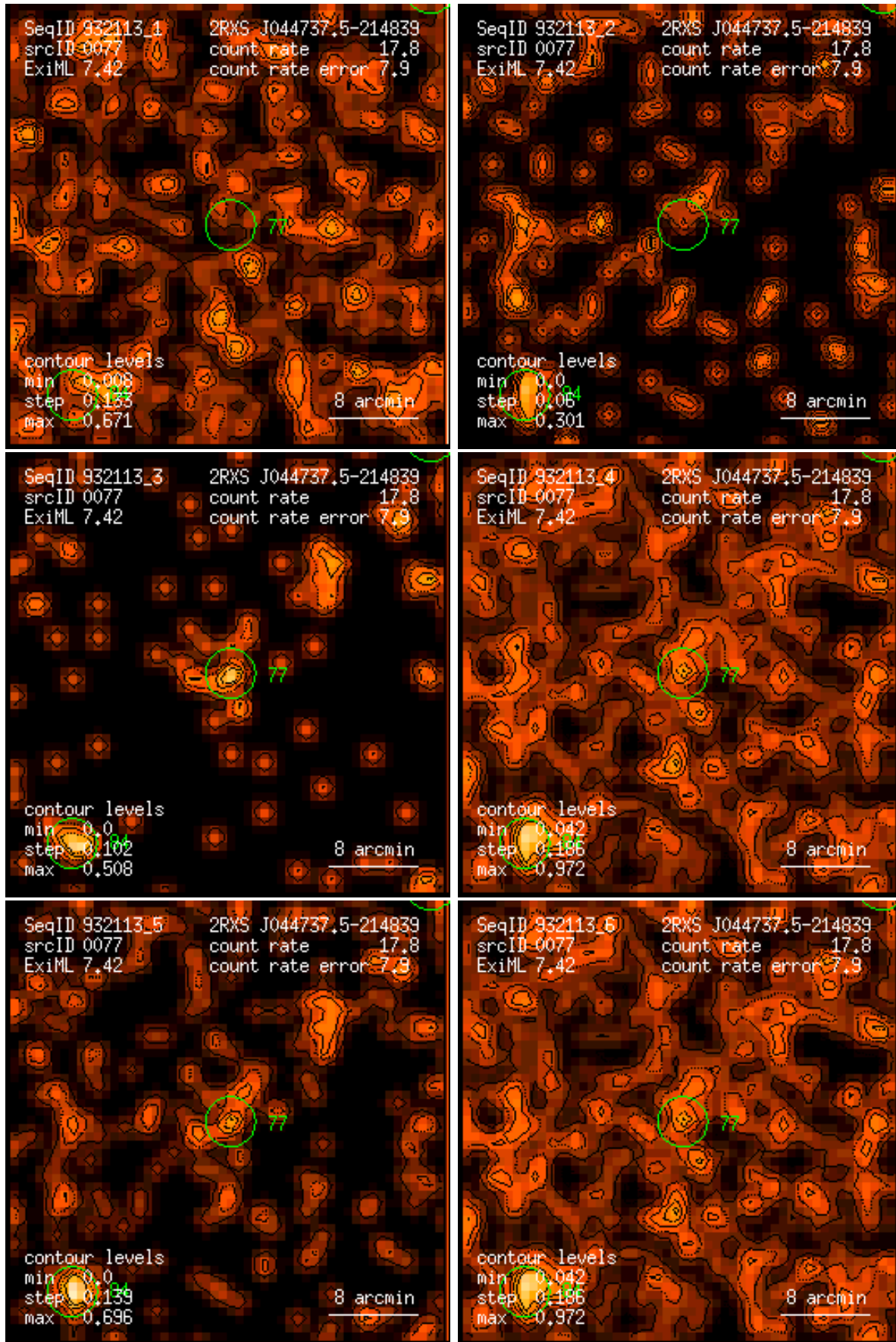
Figure 77: RASS 932113: detection 0077: band rate images, Gaussian filter: (1) PSPC channels 11 – 41, (2) 52 – 90, (3) 91 – 201, (4) 11 – 235, (5) 52 – 201, (6) 11 – 201. Broad band rates in counts/ks. Band rate contour levels in counts/ks/arcmin 2 .
