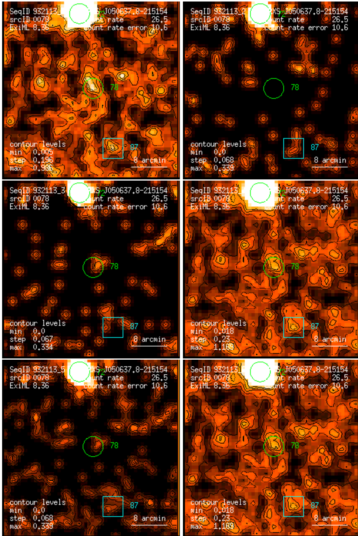
Figure 78: RASS 932113: detection 0078: band rate images, Gaussian filter: (1) PSPC channels 11 – 41, (2) 52 – 90, (3) 91 – 201, (4) 11 – 235, (5) 52 – 201, (6) 11 – 201. Broad band rates in counts/ks. Band rate contour levels in counts/ks/arcmin 2 .
