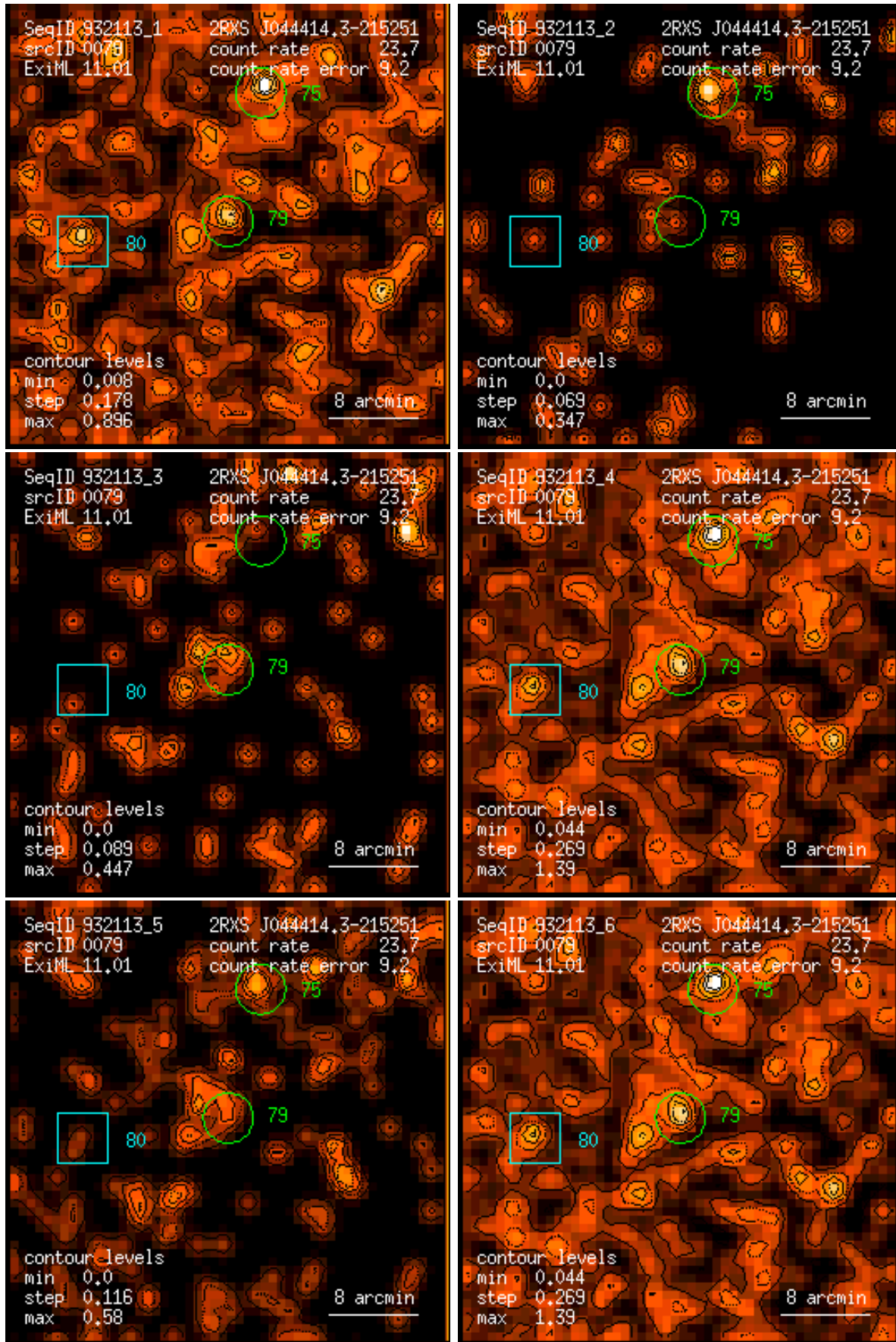
Figure 79: RASS 932113: detection 0079: band rate images, Gaussian filter: (1) PSPC channels 11 – 41, (2) 52 – 90, (3) 91 – 201, (4) 11 – 235, (5) 52 – 201, (6) 11 – 201. Broad band rates in counts/ks. Band rate contour levels in counts/ks/arcmin 2 .
