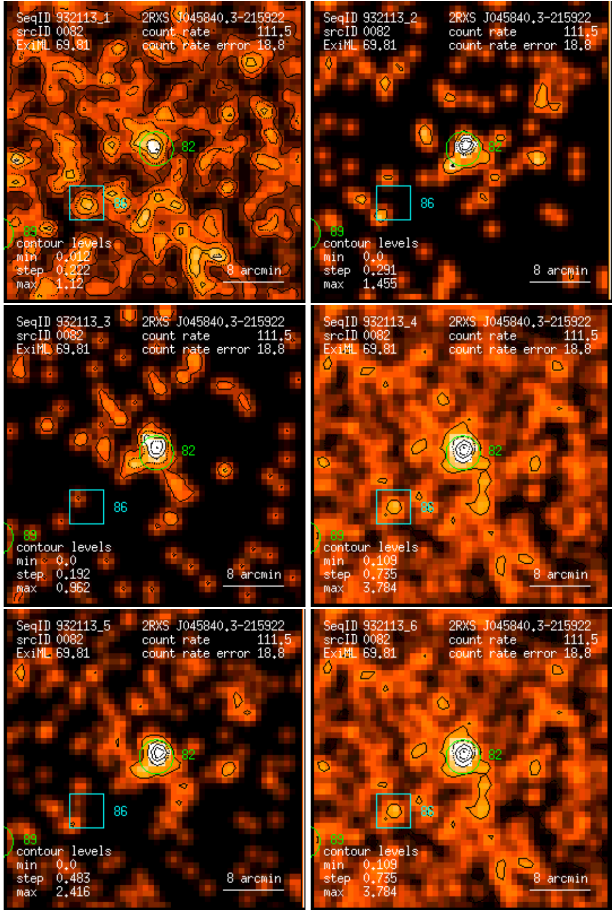
Figure 82: RASS 932113: detection 0082: band rate images, Gaussian filter: (1) PSPC channels 11 – 41, (2) 52 – 90, (3) 91 – 201, (4) 11 – 235, (5) 52 – 201, (6) 11 – 201. Broad band rates in counts/ks. Band rate contour levels in counts/ks/arcmin 2 .
