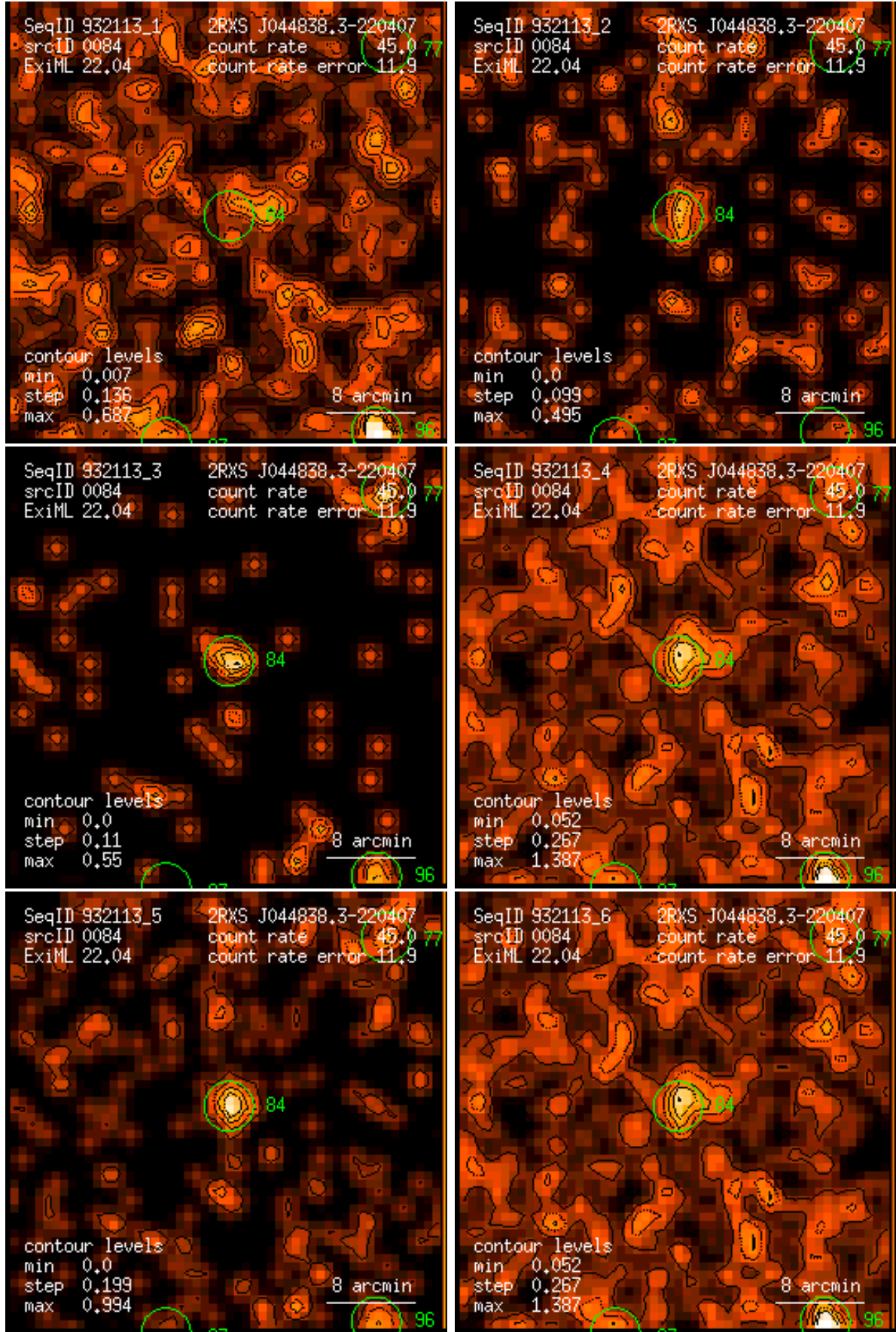
Figure 84: RASS 932113: detection 0084: band rate images, Gaussian filter: (1) PSPC channels 11 – 41, (2) 52 – 90, (3) 91 – 201, (4) 11 – 235, (5) 52 – 201, (6) 11 – 201. Broad band rates in counts/ks. Band rate contour levels in counts/ks/arcmin 2 .
