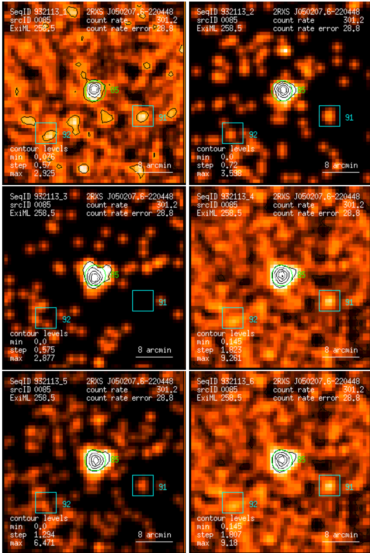
Figure 85: RASS 932113: detection 0085: band rate images, Gaussian filter: (1) PSPC channels 11 – 41, (2) 52 – 90, (3) 91 – 201, (4) 11 – 235, (5) 52 – 201, (6) 11 – 201. Broad band rates in counts/ks. Band rate contour levels in counts/ks/arcmin 2 .
