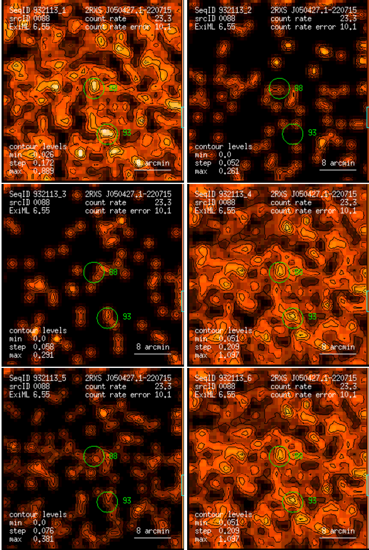
Figure 88: RASS 932113: detection 0088: band rate images, Gaussian filter: (1) PSPC channels 11 – 41, (2) 52 – 90, (3) 91 – 201, (4) 11 – 235, (5) 52 – 201, (6) 11 – 201. Broad band rates in counts/ks. Band rate contour levels in counts/ks/arcmin 2 .
