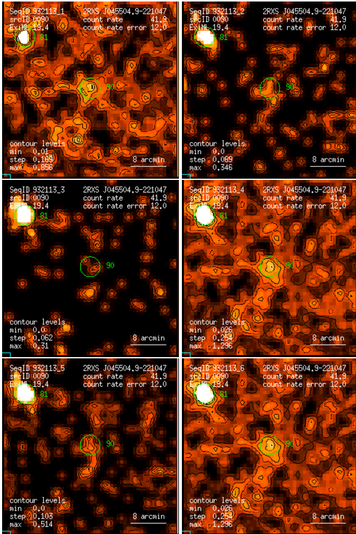
Figure 90: RASS 932113: detection 0090: band rate images, Gaussian filter: (1) PSPC channels 11 – 41, (2) 52 – 90, (3) 91 – 201, (4) 11 – 235, (5) 52 – 201, (6) 11 – 201. Broad band rates in counts/ks. Band rate contour levels in counts/ks/arcmin 2 .
