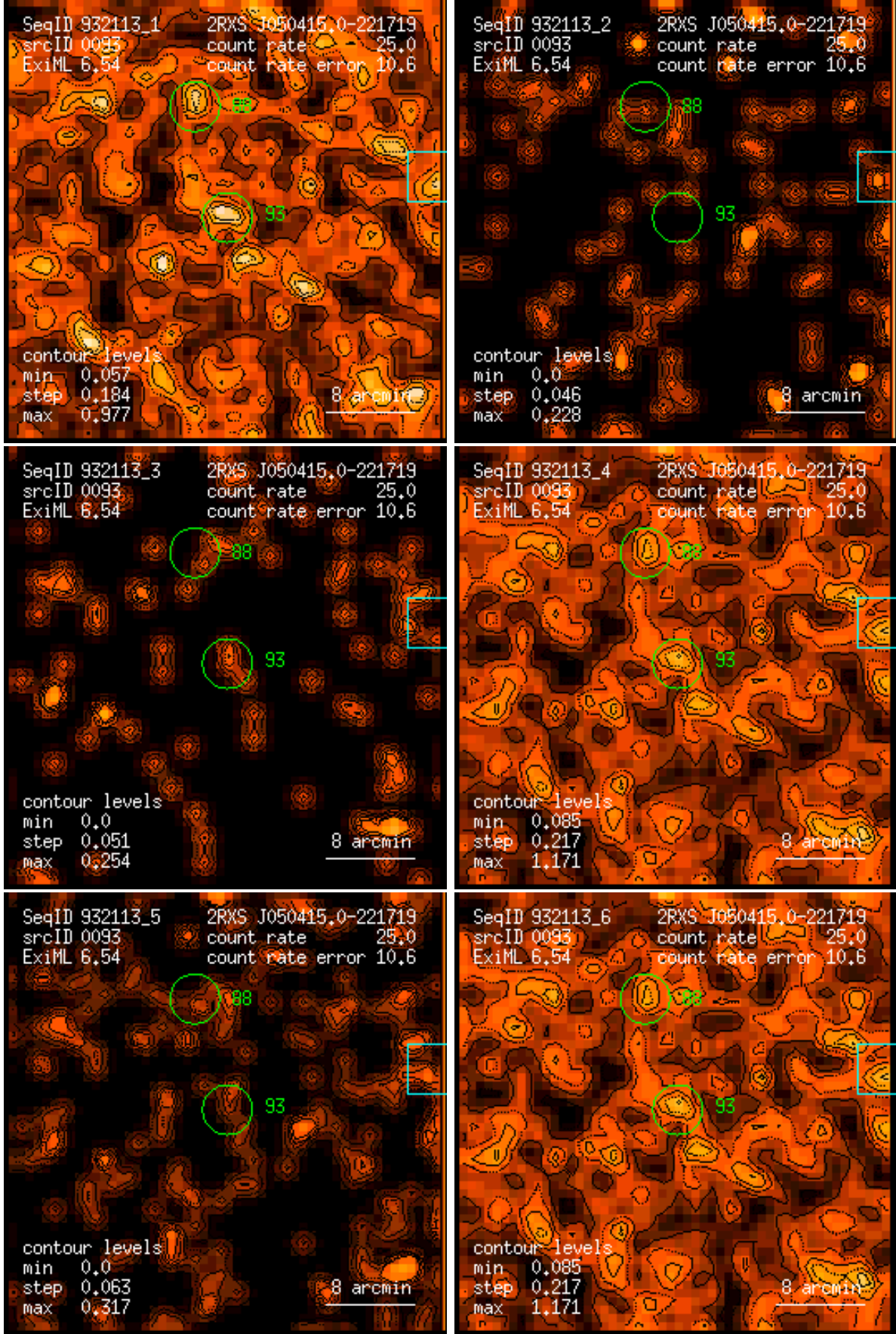
Figure 93: RASS 932113: detection 0093: band rate images, Gaussian filter: (1) PSPC channels 11 – 41, (2) 52 – 90, (3) 91 – 201, (4) 11 – 235, (5) 52 – 201, (6) 11 – 201. Broad band rates in counts/ks. Band rate contour levels in counts/ks/arcmin 2 .
