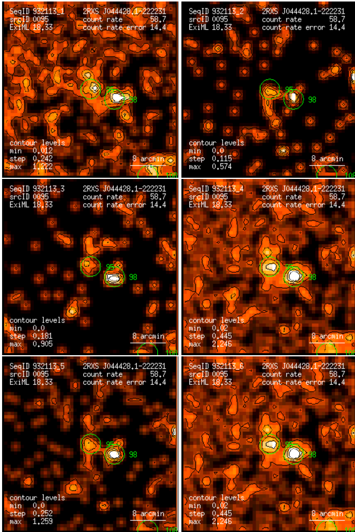
Figure 95: RASS 932113: detection 0095: band rate images, Gaussian filter: (1) PSPC channels 11 – 41, (2) 52 – 90, (3) 91 – 201, (4) 11 – 235, (5) 52 – 201, (6) 11 – 201. Broad band rates in counts/ks. Band rate contour levels in counts/ks/arcmin 2 .
