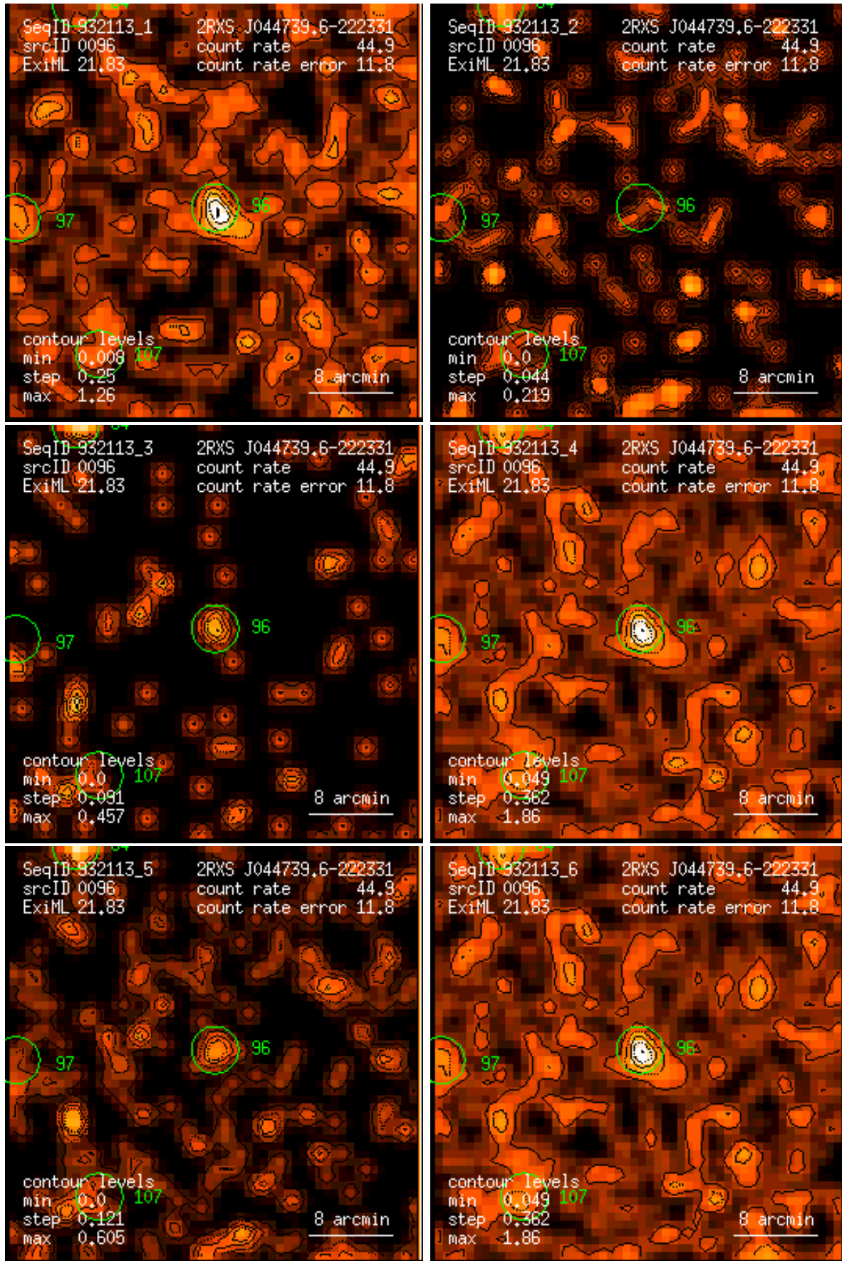
Figure 96: RASS 932113: detection 0096: band rate images, Gaussian filter: (1) PSPC channels 11 – 41, (2) 52 – 90, (3) 91 – 201, (4) 11 – 235, (5) 52 – 201, (6) 11 – 201. Broad band rates in counts/ks. Band rate contour levels in counts/ks/arcmin 2 .
