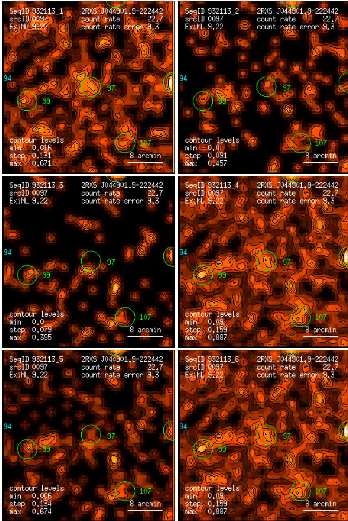
Figure 97: RASS 932113: detection 0097: band rate images, Gaussian filter: (1) PSPC channels 11 – 41, (2) 52 – 90, (3) 91 – 201, (4) 11 – 235, (5) 52 – 201, (6) 11 – 201. Broad band rates in counts/ks. Band rate contour levels in counts/ks/arcmin 2 .
