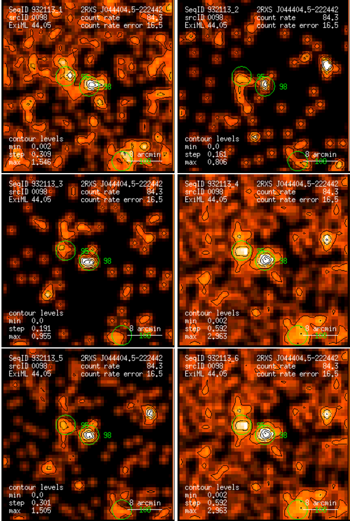
Figure 98: RASS 932113: detection 0098: band rate images, Gaussian filter: (1) PSPC channels 11 – 41, (2) 52 – 90, (3) 91 – 201, (4) 11 – 235, (5) 52 – 201, (6) 11 – 201. Broad band rates in counts/ks. Band rate contour levels in counts/ks/arcmin 2 .
