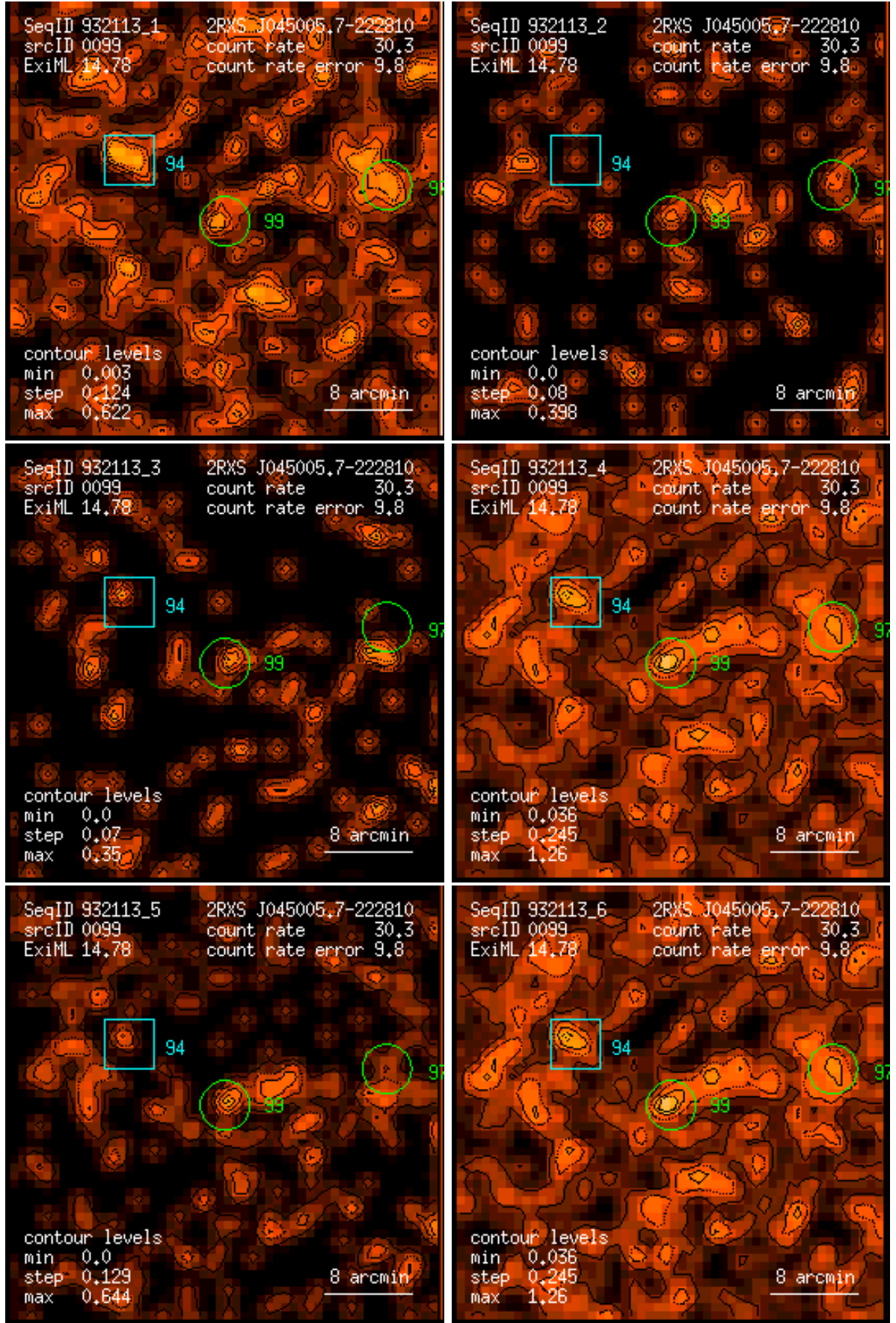
Figure 99: RASS 932113: detection 0099: band rate images, Gaussian filter: (1) PSPC channels 11 – 41, (2) 52 – 90, (3) 91 – 201, (4) 11 – 235, (5) 52 – 201, (6) 11 – 201. Broad band rates in counts/ks. Band rate contour levels in counts/ks/arcmin 2 .
