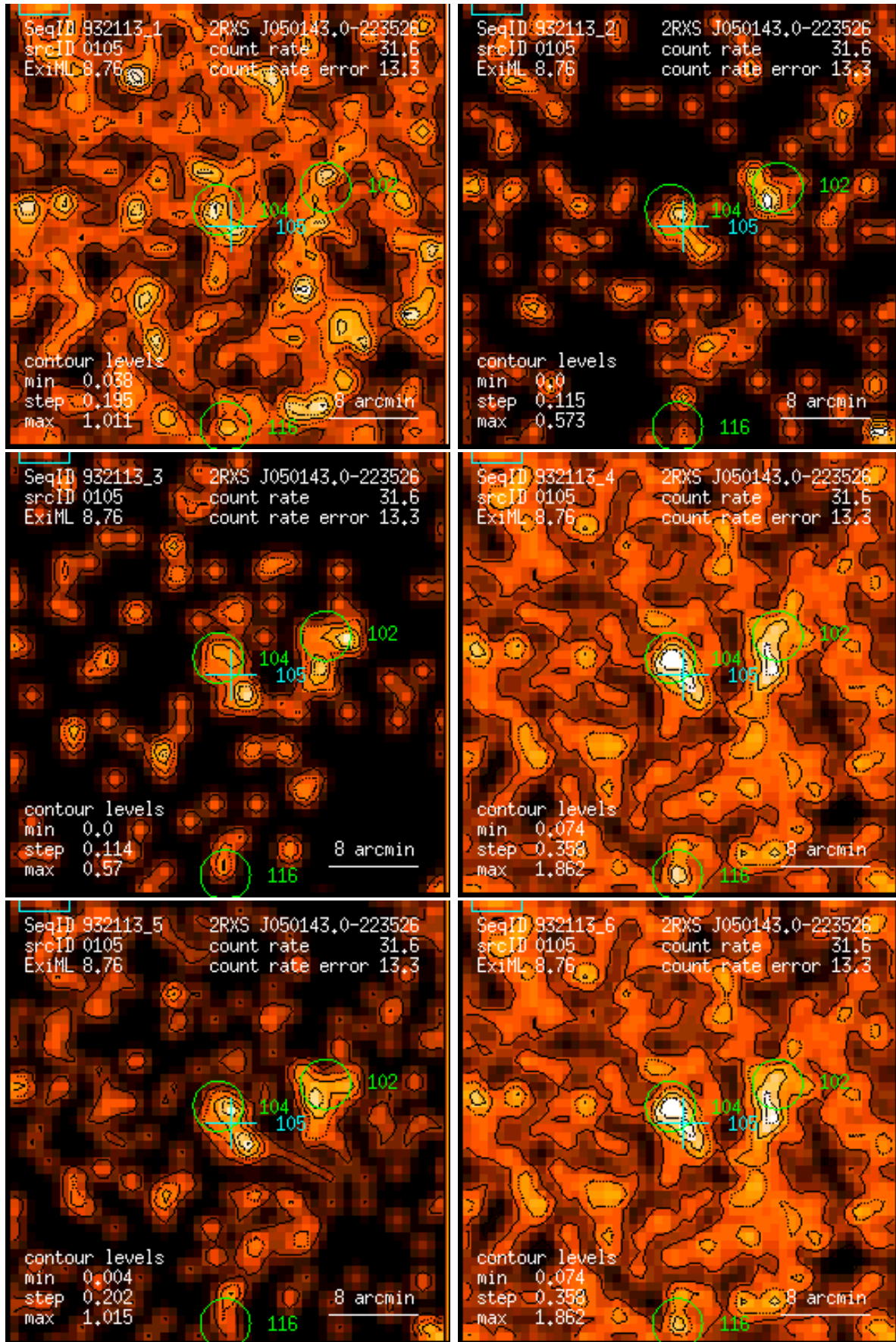
Figure 105: RASS 932113: detection 0105: band rate images, Gaussian filter: (1) PSPC channels 11 – 41, (2) 52 – 90, (3) 91 – 201, (4) 11 – 235, (5) 52 – 201, (6) 11 – 201. Broad band rates in counts/ks. Band rate contour levels in counts/ks/arcmin 2 .
