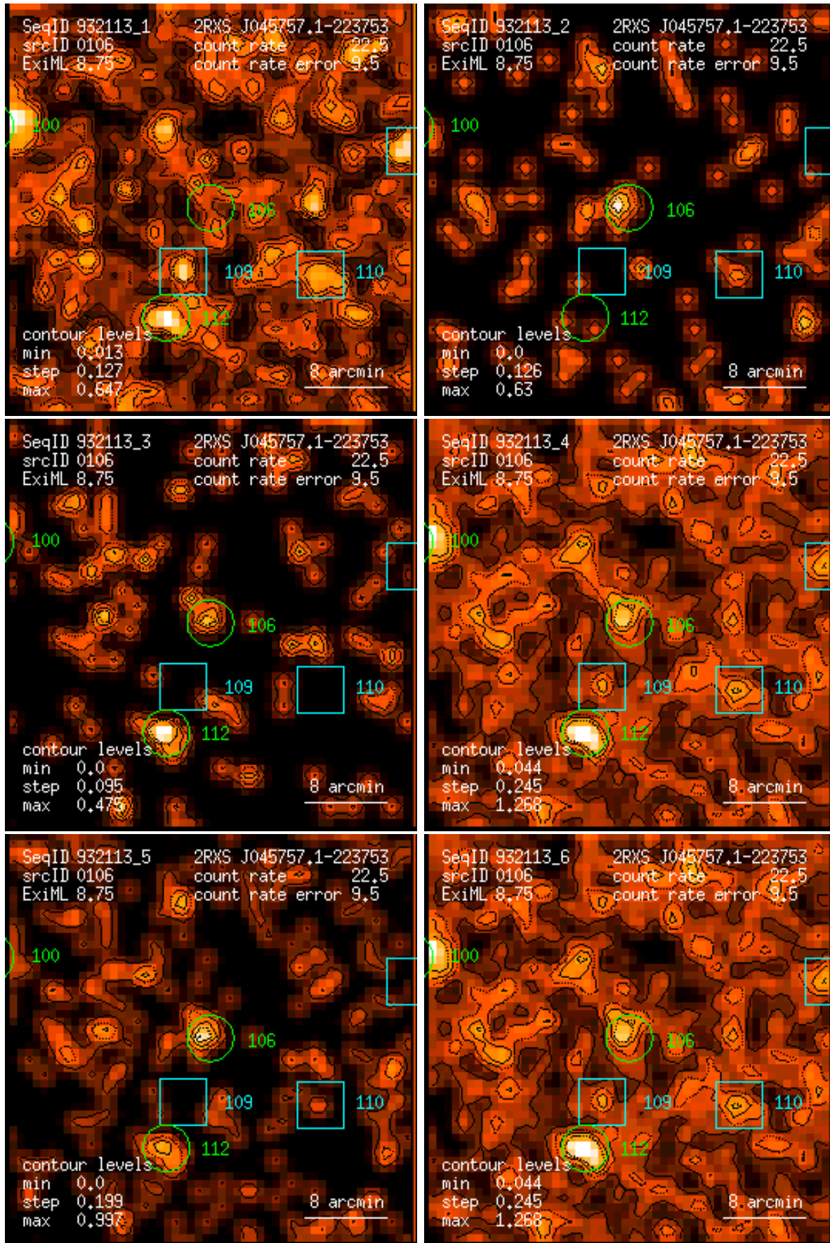
Figure 106: RASS 932113: detection 0106: band rate images, Gaussian filter: (1) PSPC channels 11 – 41, (2) 52 – 90, (3) 91 – 201, (4) 11 – 235, (5) 52 – 201, (6) 11 – 201. Broad band rates in counts/ks. Band rate contour levels in counts/ks/arcmin 2 .
