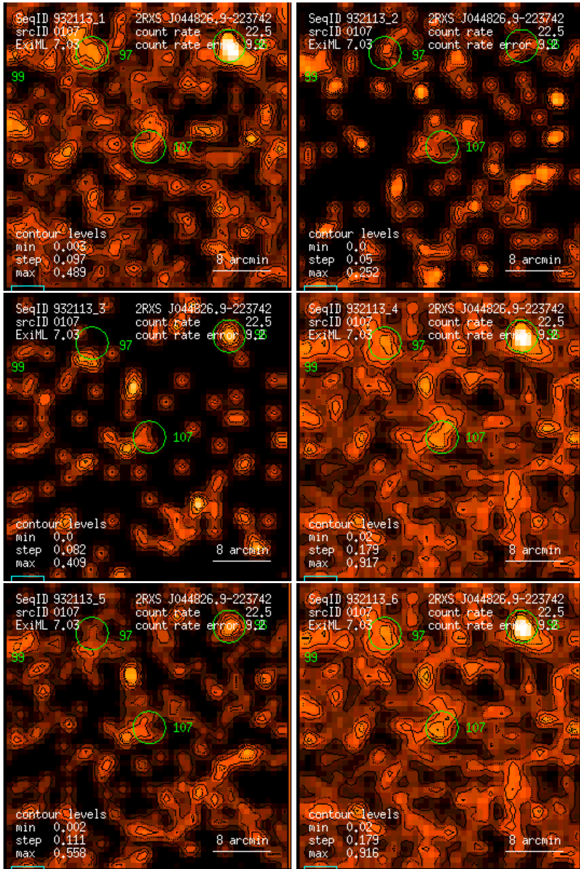
Figure 107: RASS 932113: detection 0107: band rate images, Gaussian filter: (1) PSPC channels 11 – 41, (2) 52 – 90, (3) 91 – 201, (4) 11 – 235, (5) 52 – 201, (6) 11 – 201. Broad band rates in counts/ks. Band rate contour levels in counts/ks/arcmin 2 .
