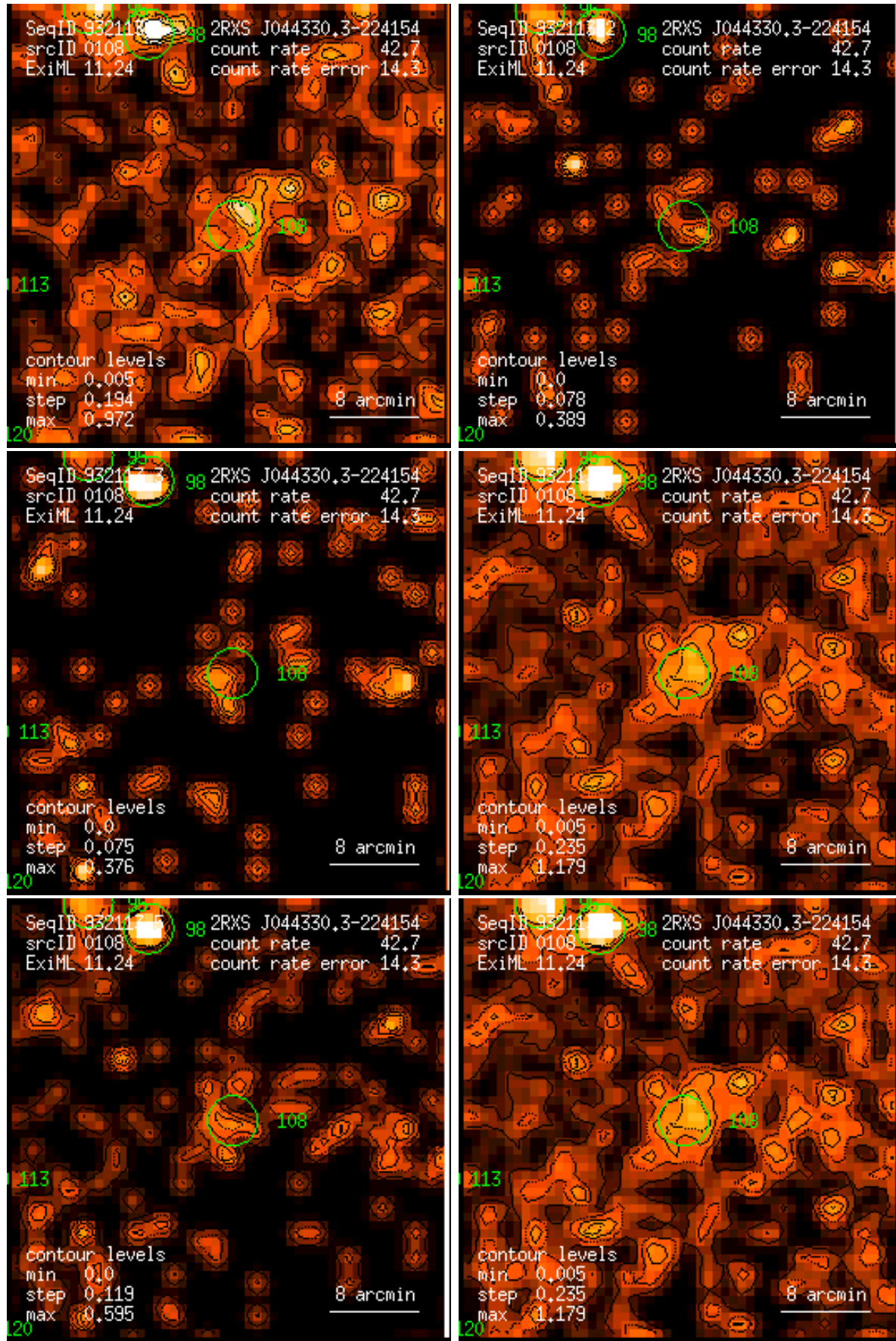
Figure 108: RASS 932113: detection 0108: band rate images, Gaussian filter: (1) PSPC channels 11 – 41, (2) 52 – 90, (3) 91 – 201, (4) 11 – 235, (5) 52 – 201, (6) 11 – 201. Broad band rates in counts/ks. Band rate contour levels in counts/ks/arcmin 2 .
