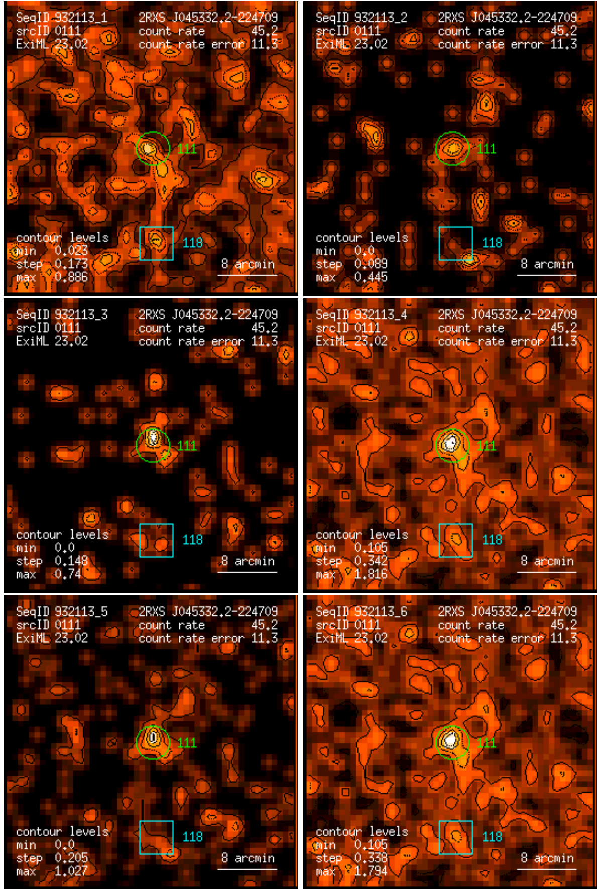
Figure 111: RASS 932113: detection 0111: band rate images, Gaussian filter: (1) PSPC channels 11 – 41, (2) 52 – 90, (3) 91 – 201, (4) 11 – 235, (5) 52 – 201, (6) 11 – 201. Broad band rates in counts/ks. Band rate contour levels in counts/ks/arcmin 2 .
