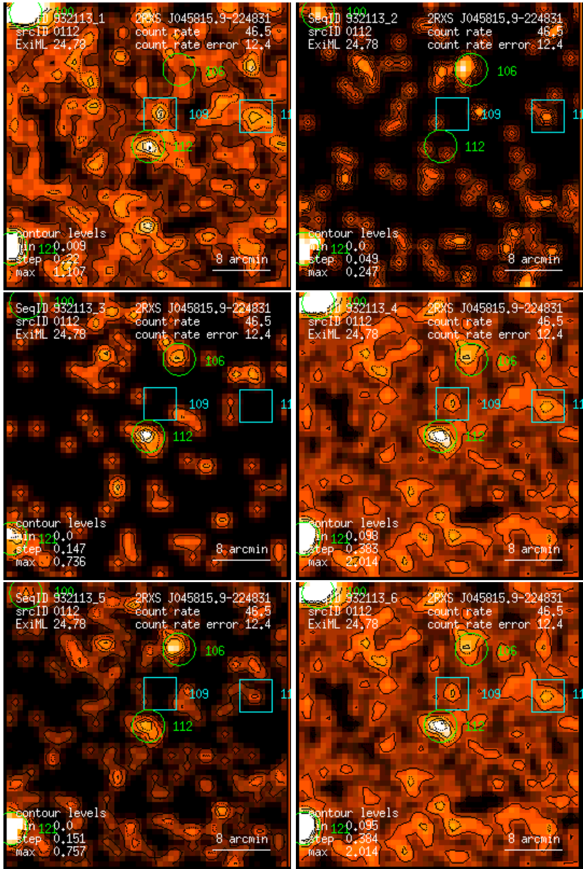
Figure 112: RASS 932113: detection 0112: band rate images, Gaussian filter: (1) PSPC channels 11 – 41, (2) 52 – 90, (3) 91 – 201, (4) 11 – 235, (5) 52 – 201, (6) 11 – 201. Broad band rates in counts/ks. Band rate contour levels in counts/ks/arcmin 2 .
