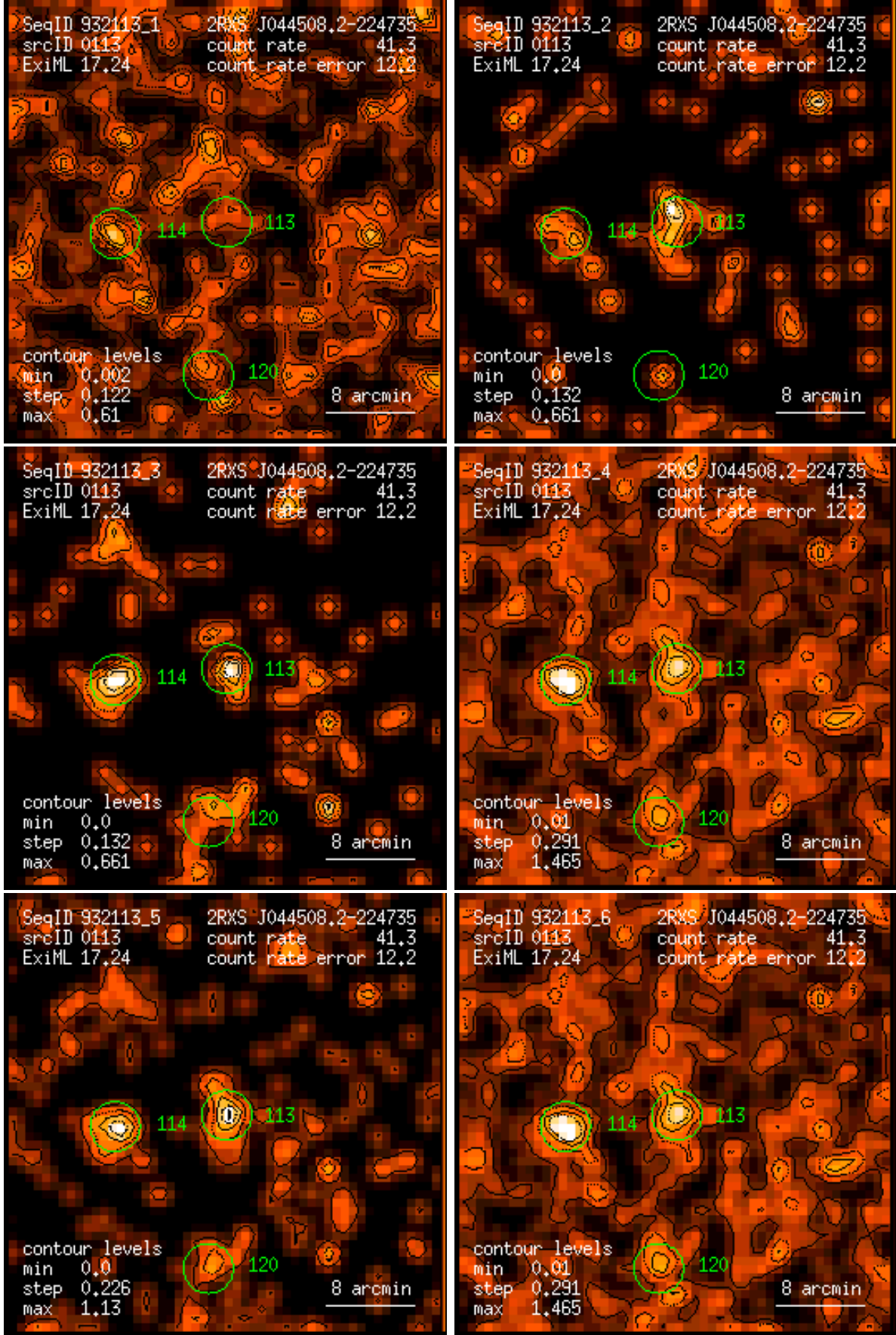
Figure 113: RASS 932113: detection 0113: band rate images, Gaussian filter: (1) PSPC channels 11 – 41, (2) 52 – 90, (3) 91 – 201, (4) 11 – 235, (5) 52 – 201, (6) 11 – 201. Broad band rates in counts/ks. Band rate contour levels in counts/ks/arcmin 2 .
