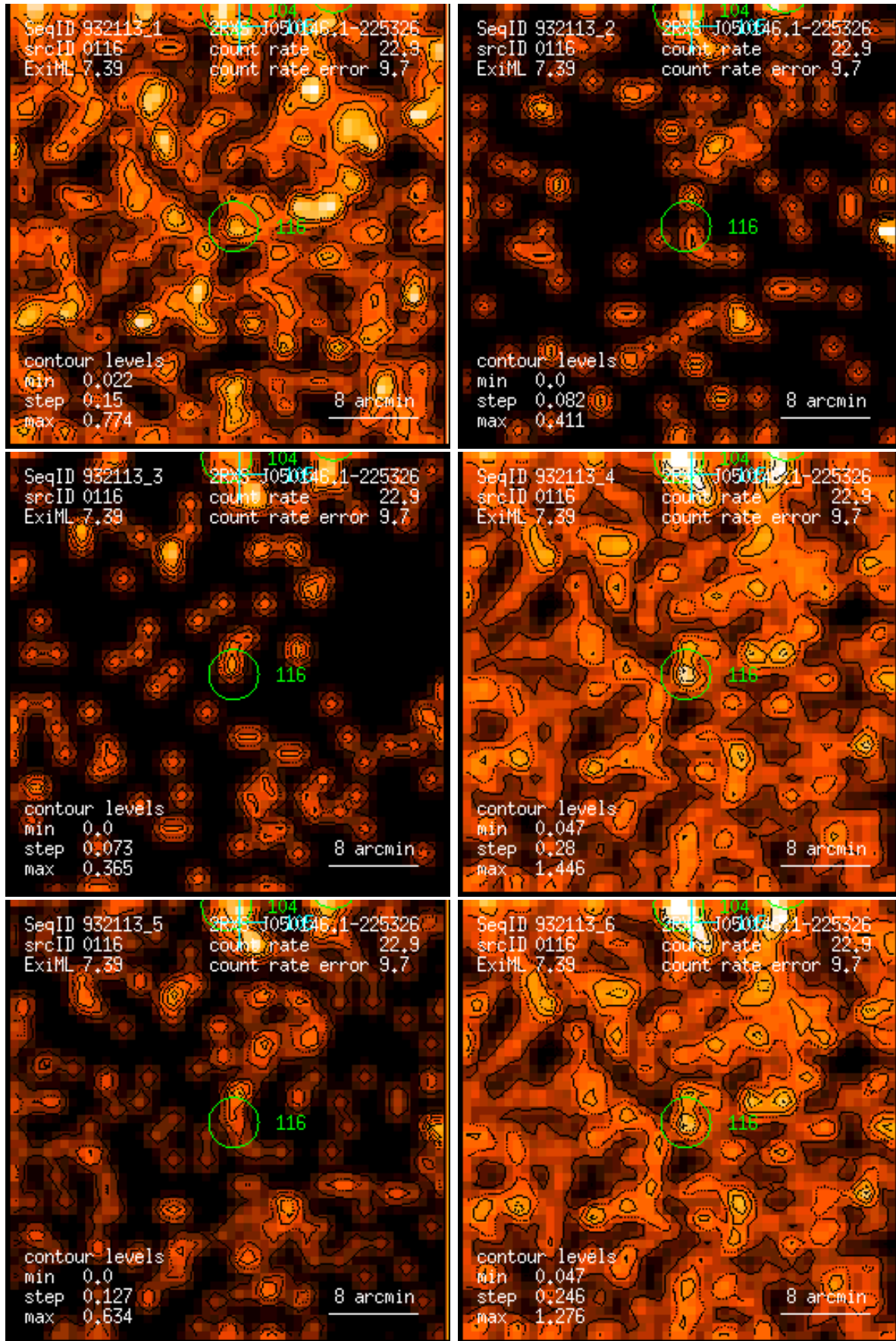
Figure 116: RASS 932113: detection 0116: band rate images, Gaussian filter: (1) PSPC channels 11 – 41, (2) 52 – 90, (3) 91 – 201, (4) 11 – 235, (5) 52 – 201, (6) 11 – 201. Broad band rates in counts/ks. Band rate contour levels in counts/ks/arcmin 2 .
