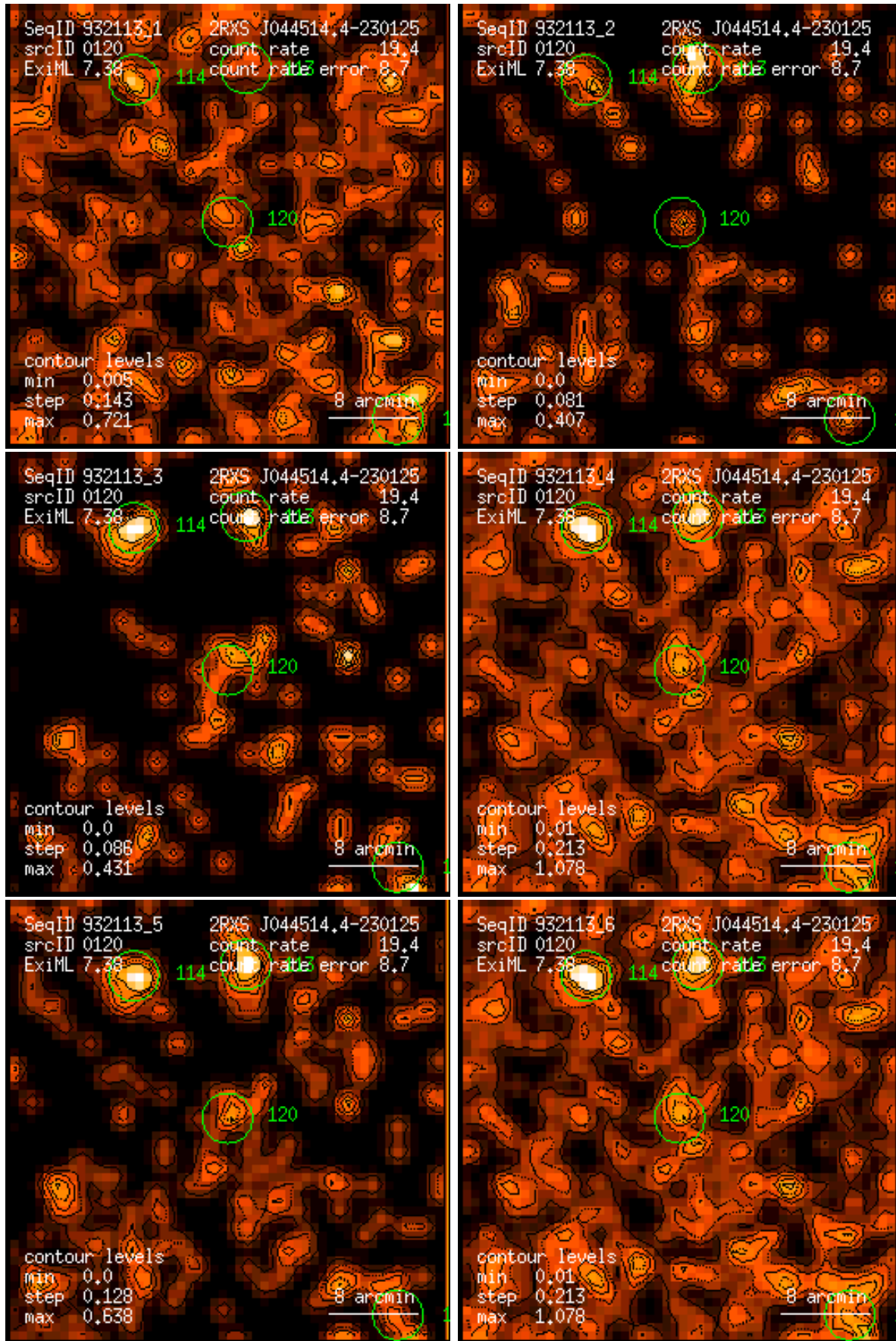
Figure 120: RASS 932113: detection 0120: band rate images, Gaussian filter: (1) PSPC channels 11 – 41, (2) 52 – 90, (3) 91 – 201, (4) 11 – 235, (5) 52 – 201, (6) 11 – 201. Broad band rates in counts/ks. Band rate contour levels in counts/ks/arcmin 2 .
