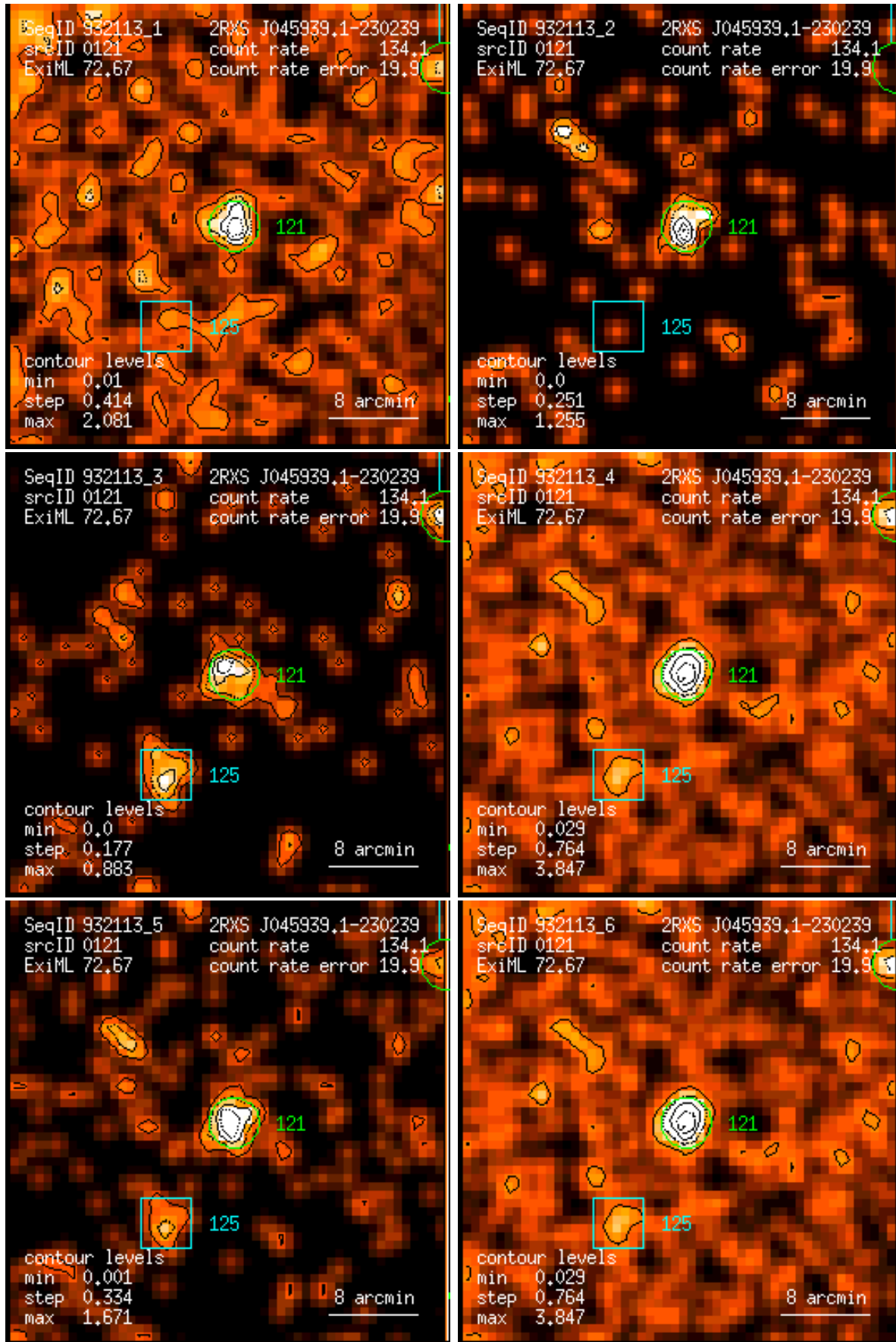
Figure 121: RASS 932113: detection 0121: band rate images, Gaussian filter: (1) PSPC channels 11 – 41, (2) 52 – 90, (3) 91 – 201, (4) 11 – 235, (5) 52 – 201, (6) 11 – 201. Broad band rates in counts/ks. Band rate contour levels in counts/ks/arcmin 2 .
