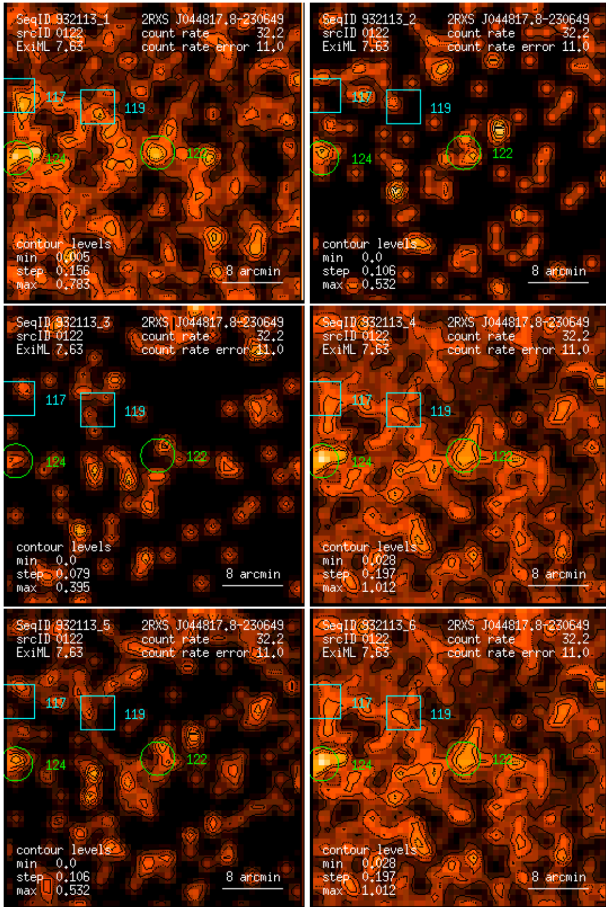
Figure 122: RASS 932113: detection 0122: band rate images, Gaussian filter: (1) PSPC channels 11 – 41, (2) 52 – 90, (3) 91 – 201, (4) 11 – 235, (5) 52 – 201, (6) 11 – 201. Broad band rates in counts/ks. Band rate contour levels in counts/ks/arcmin 2 .
