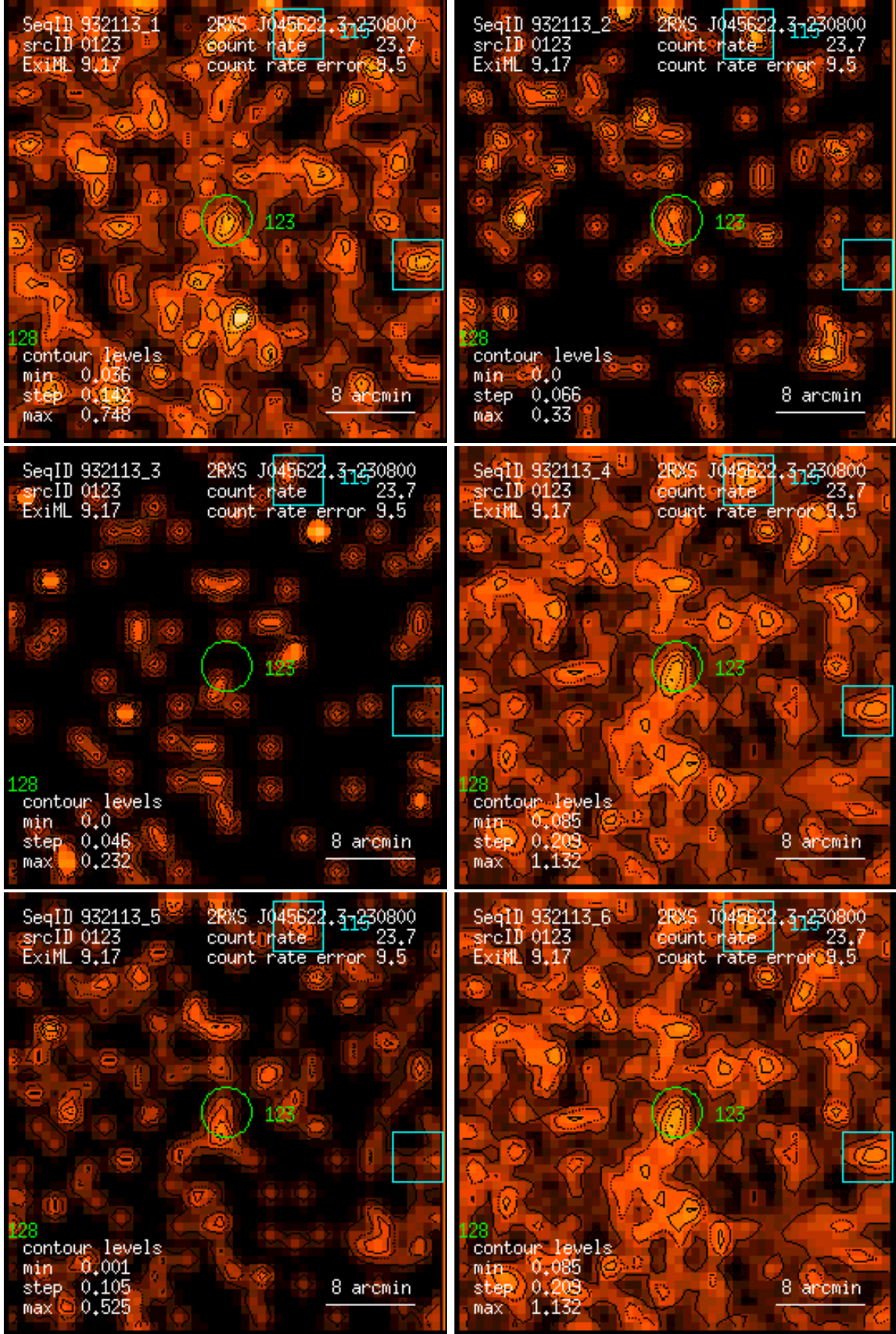
Figure 123: RASS 932113: detection 0123: band rate images, Gaussian filter: (1) PSPC channels 11 – 41, (2) 52 – 90, (3) 91 – 201, (4) 11 – 235, (5) 52 – 201, (6) 11 – 201. Broad band rates in counts/ks. Band rate contour levels in counts/ks/arcmin 2 .
