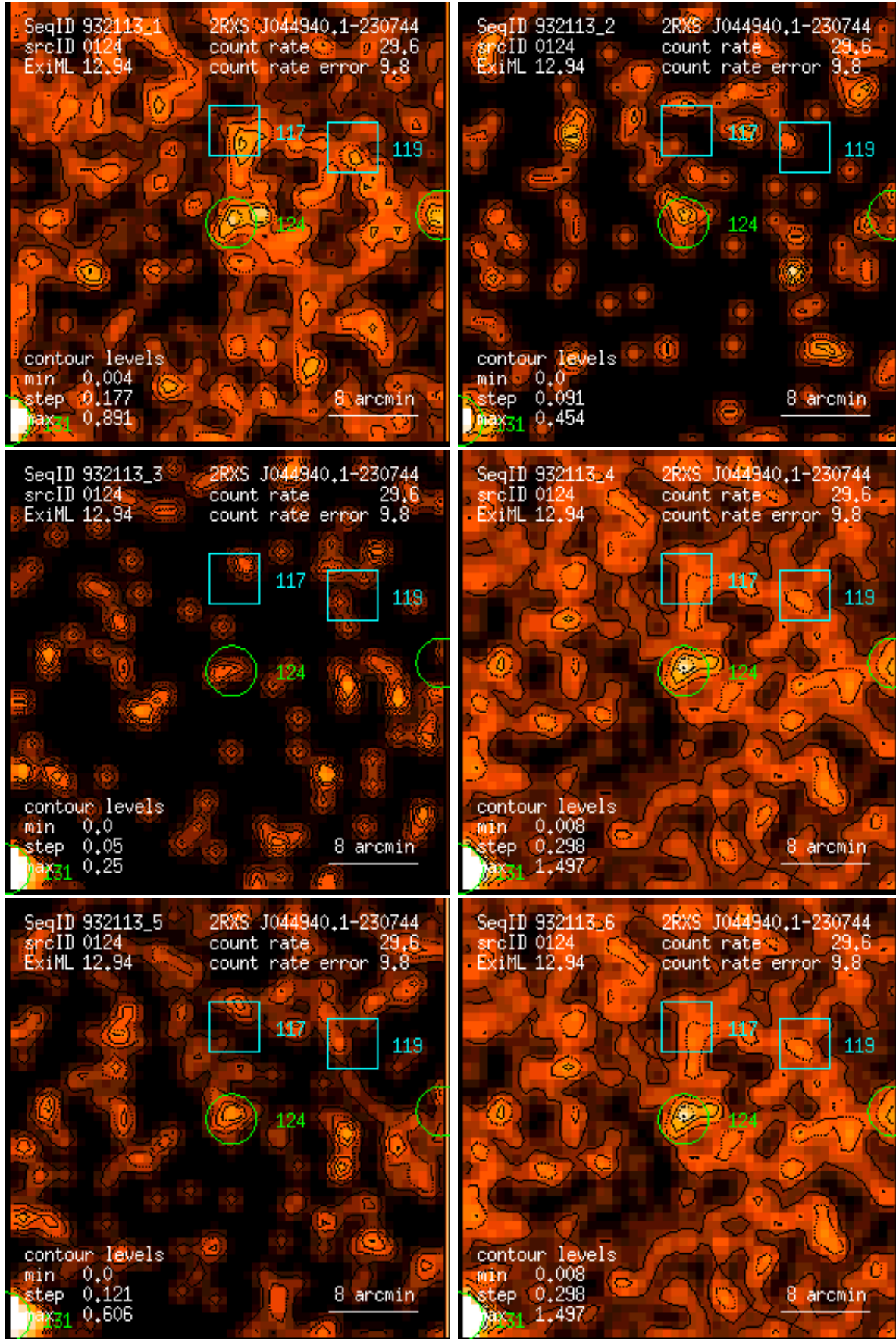
Figure 124: RASS 932113: detection 0124: band rate images, Gaussian filter: (1) PSPC channels 11 – 41, (2) 52 – 90, (3) 91 – 201, (4) 11 – 235, (5) 52 – 201, (6) 11 – 201. Broad band rates in counts/ks. Band rate contour levels in counts/ks/arcmin 2 .
