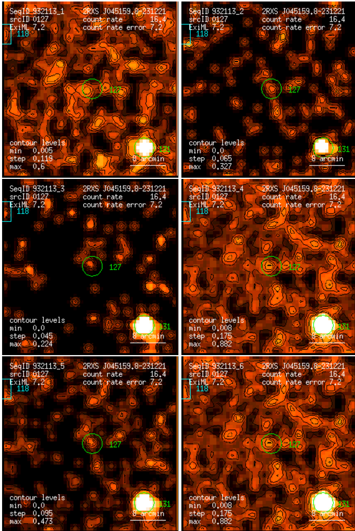
Figure 127: RASS 932113: detection 0127: band rate images, Gaussian filter: (1) PSPC channels 11 – 41, (2) 52 – 90, (3) 91 – 201, (4) 11 – 235, (5) 52 – 201, (6) 11 – 201. Broad band rates in counts/ks. Band rate contour levels in counts/ks/arcmin 2 .
