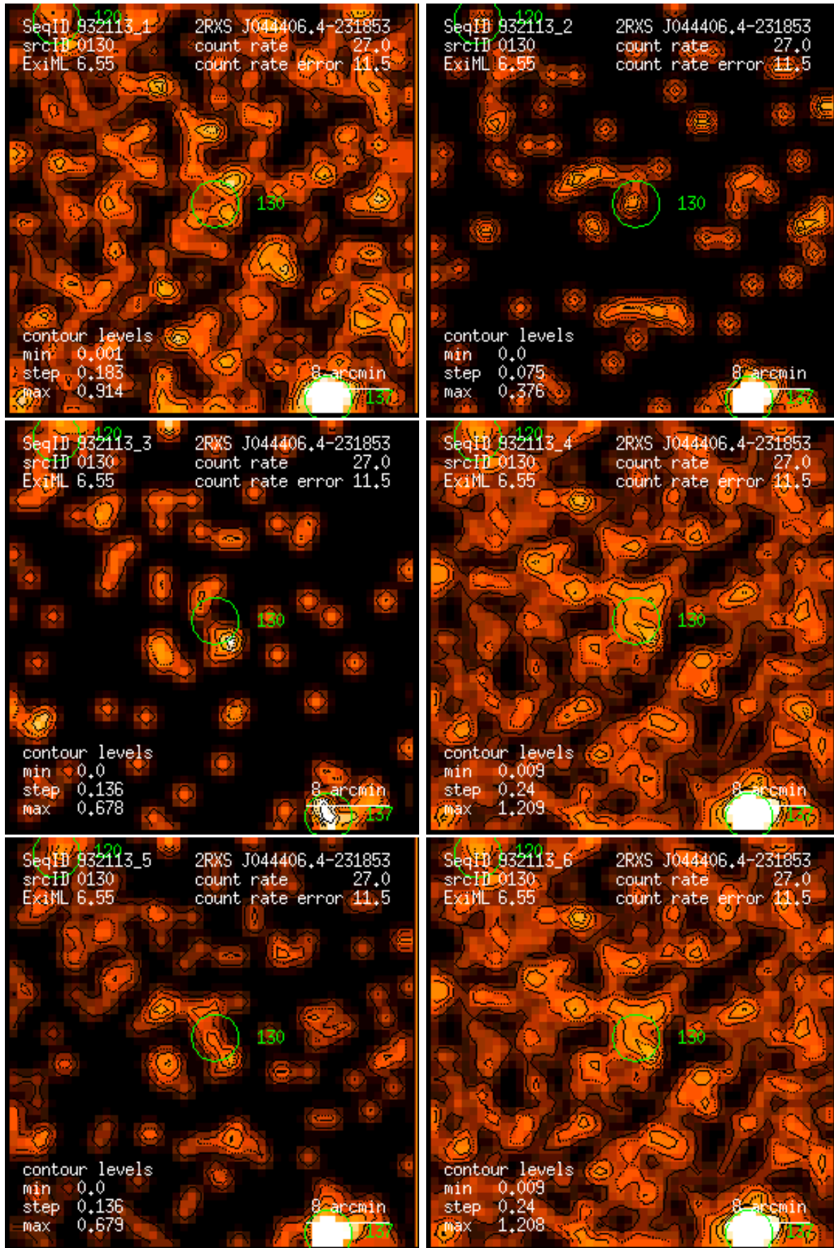
Figure 130: RASS 932113: detection 0130: band rate images, Gaussian filter: (1) PSPC channels 11 – 41, (2) 52 – 90, (3) 91 – 201, (4) 11 – 235, (5) 52 – 201, (6) 11 – 201. Broad band rates in counts/ks. Band rate contour levels in counts/ks/arcmin 2 .
