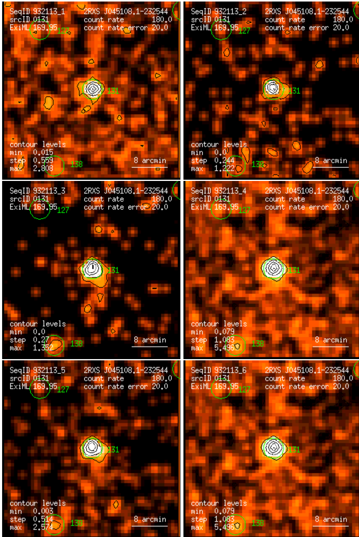
Figure 131: RASS 932113: detection 0131: band rate images, Gaussian filter: (1) PSPC channels 11 – 41, (2) 52 – 90, (3) 91 – 201, (4) 11 – 235, (5) 52 – 201, (6) 11 – 201. Broad band rates in counts/ks. Band rate contour levels in counts/ks/arcmin 2 .
