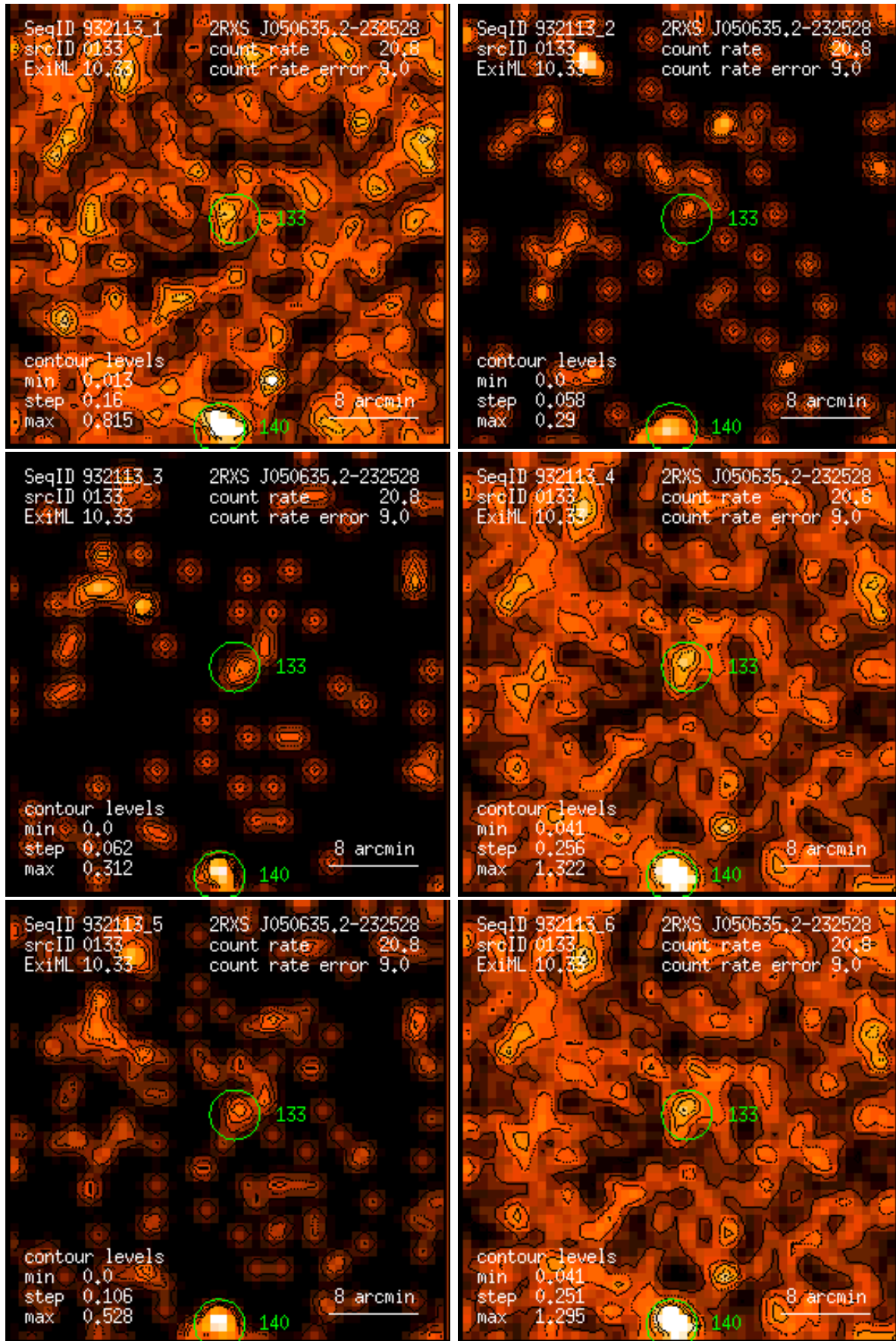
Figure 133: RASS 932113: detection 0133: band rate images, Gaussian filter: (1) PSPC channels 11 – 41, (2) 52 – 90, (3) 91 – 201, (4) 11 – 235, (5) 52 – 201, (6) 11 – 201. Broad band rates in counts/ks. Band rate contour levels in counts/ks/arcmin 2 .
