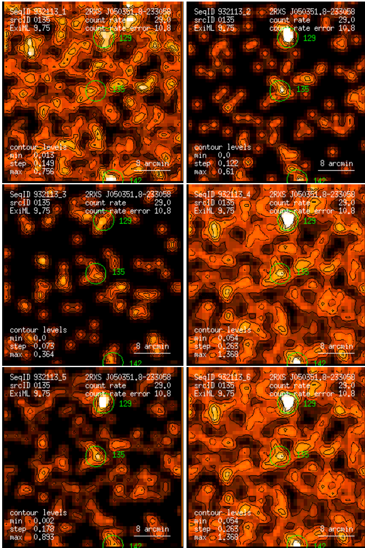
Figure 135: RASS 932113: detection 0135: band rate images, Gaussian filter: (1) PSPC channels 11 – 41, (2) 52 – 90, (3) 91 – 201, (4) 11 – 235, (5) 52 – 201, (6) 11 – 201. Broad band rates in counts/ks. Band rate contour levels in counts/ks/arcmin 2 .
