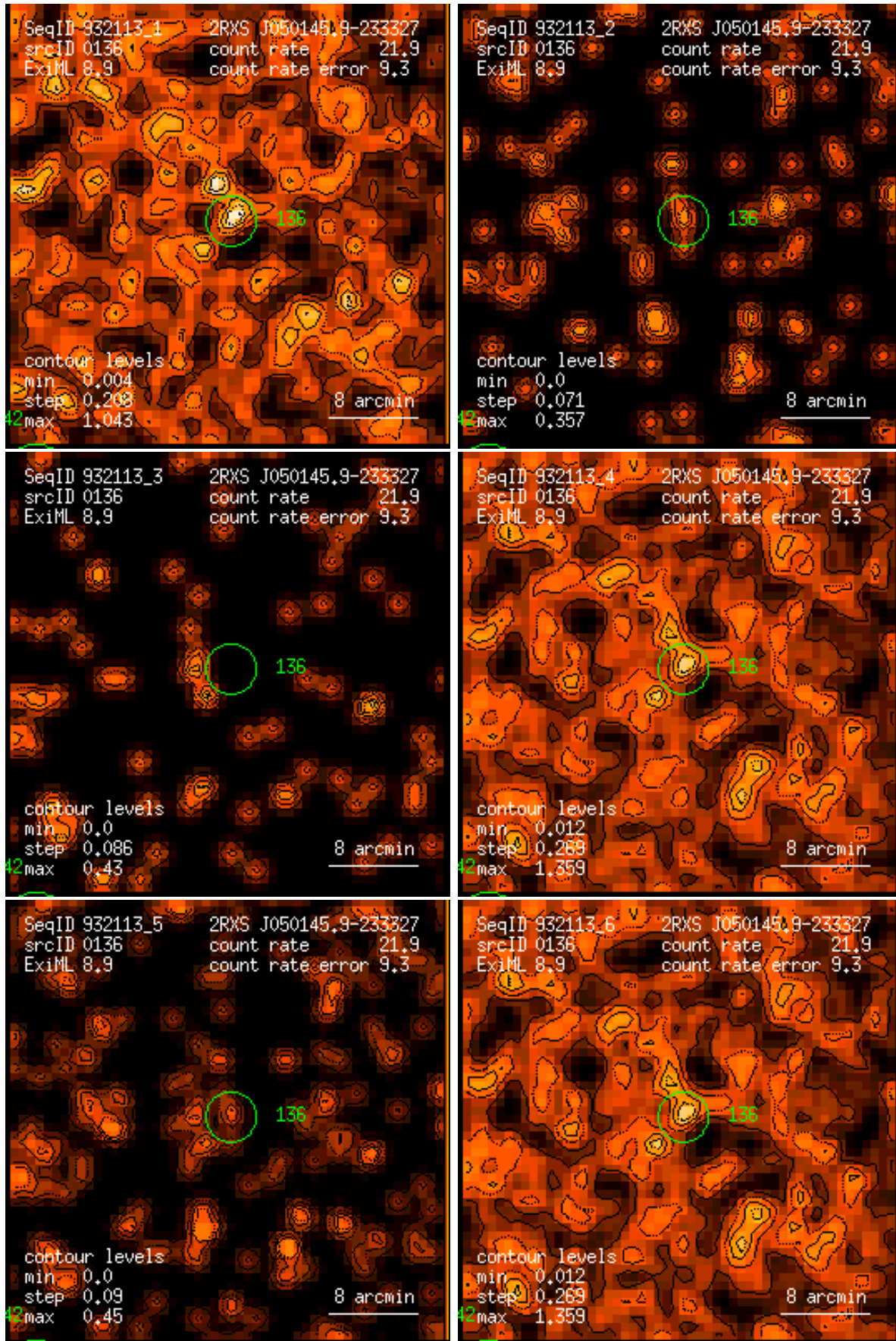
Figure 136: RASS 932113: detection 0136: band rate images, Gaussian filter: (1) PSPC channels 11 – 41, (2) 52 – 90, (3) 91 – 201, (4) 11 – 235, (5) 52 – 201, (6) 11 – 201. Broad band rates in counts/ks. Band rate contour levels in counts/ks/arcmin 2 .
