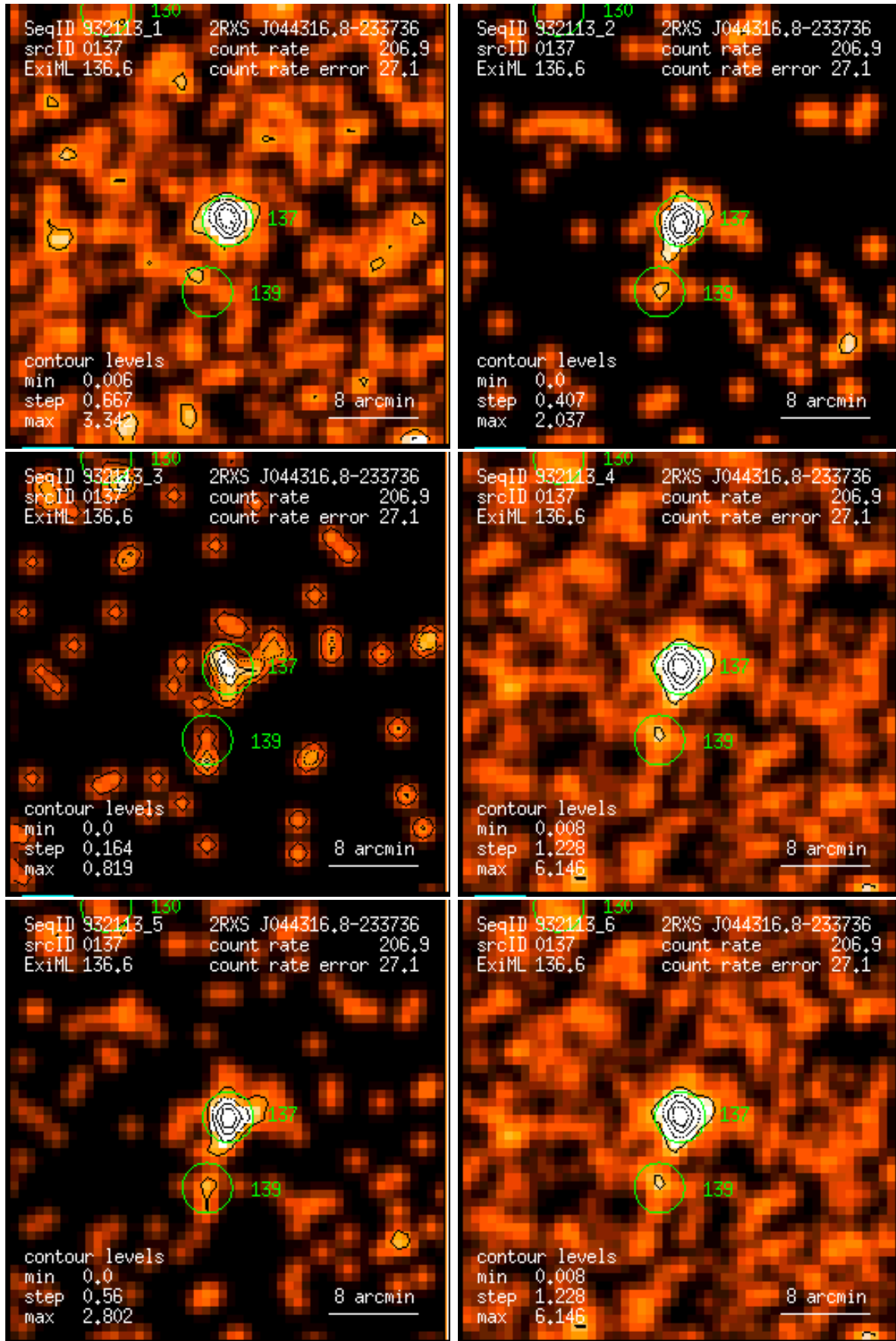
Figure 137: RASS 932113: detection 0137: band rate images, Gaussian filter: (1) PSPC channels 11 – 41, (2) 52 – 90, (3) 91 – 201, (4) 11 – 235, (5) 52 – 201, (6) 11 – 201. Broad band rates in counts/ks. Band rate contour levels in counts/ks/arcmin 2 .
