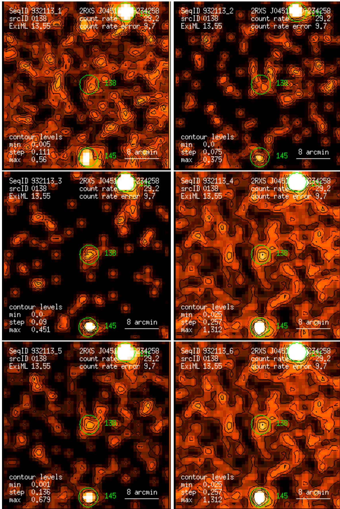
Figure 138: RASS 932113: detection 0138: band rate images, Gaussian filter: (1) PSPC channels 11 – 41, (2) 52 – 90, (3) 91 – 201, (4) 11 – 235, (5) 52 – 201, (6) 11 – 201. Broad band rates in counts/ks. Band rate contour levels in counts/ks/arcmin 2 .
