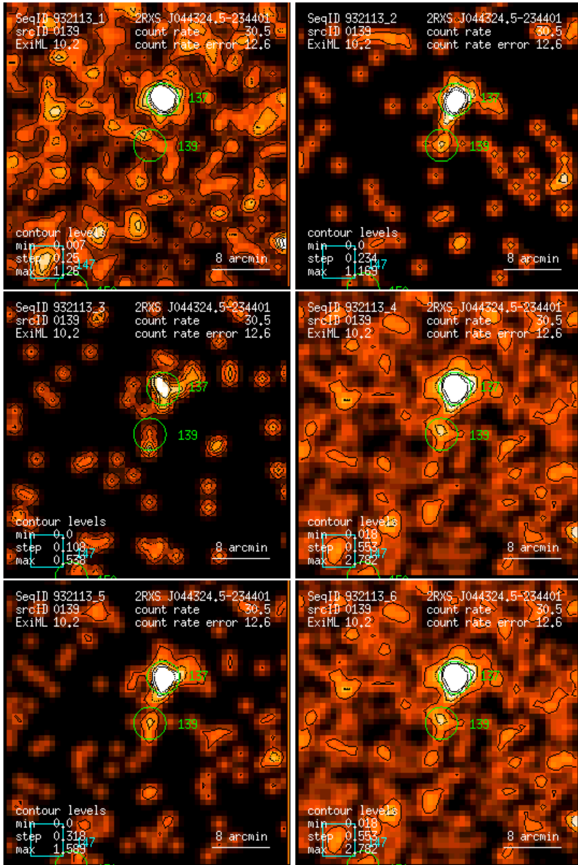
Figure 139: RASS 932113: detection 0139: band rate images, Gaussian filter: (1) PSPC channels 11 – 41, (2) 52 – 90, (3) 91 – 201, (4) 11 – 235, (5) 52 – 201, (6) 11 – 201. Broad band rates in counts/ks. Band rate contour levels in counts/ks/arcmin 2 .
