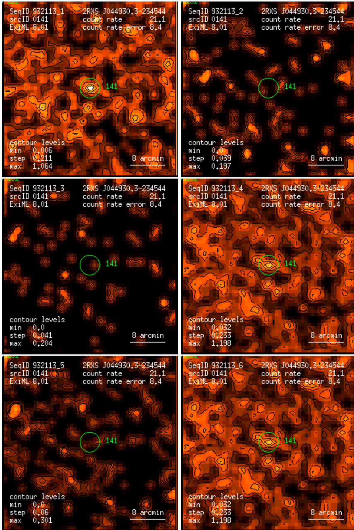
Figure 141: RASS 932113: detection 0141: band rate images, Gaussian filter: (1) PSPC channels 11 – 41, (2) 52 – 90, (3) 91 – 201, (4) 11 – 235, (5) 52 – 201, (6) 11 – 201. Broad band rates in counts/ks. Band rate contour levels in counts/ks/arcmin 2 .
