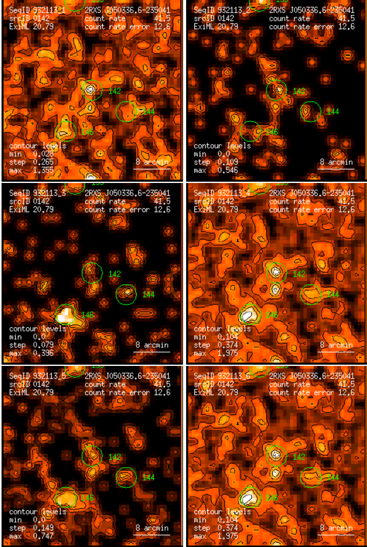
Figure 142: RASS 932113: detection 0142: band rate images, Gaussian filter: (1) PSPC channels 11 – 41, (2) 52 – 90, (3) 91 – 201, (4) 11 – 235, (5) 52 – 201, (6) 11 – 201. Broad band rates in counts/ks. Band rate contour levels in counts/ks/arcmin 2 .
