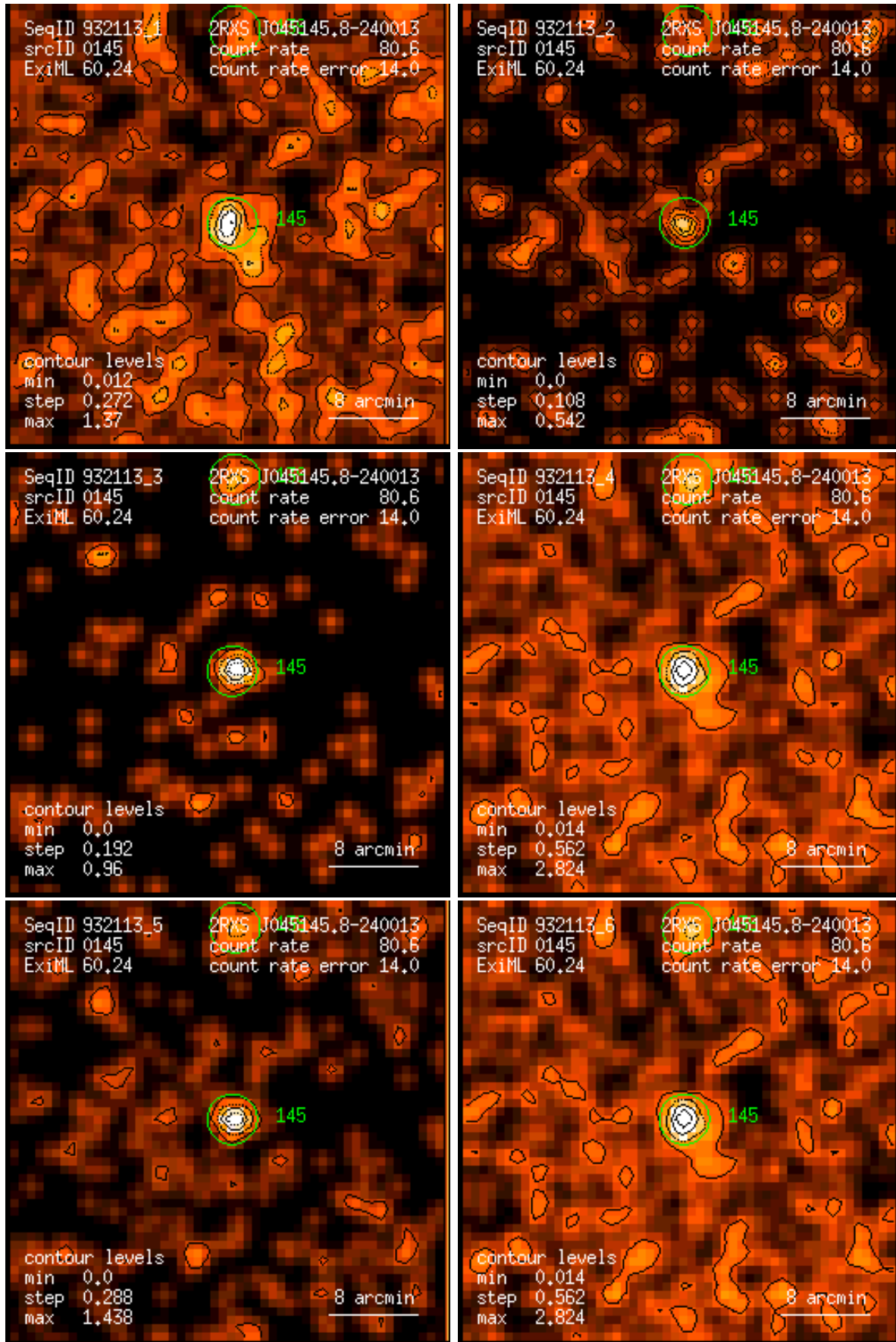
Figure 145: RASS 932113: detection 0145: band rate images, Gaussian filter: (1) PSPC channels 11 – 41, (2) 52 – 90, (3) 91 – 201, (4) 11 – 235, (5) 52 – 201, (6) 11 – 201. Broad band rates in counts/ks. Band rate contour levels in counts/ks/arcmin 2 .
