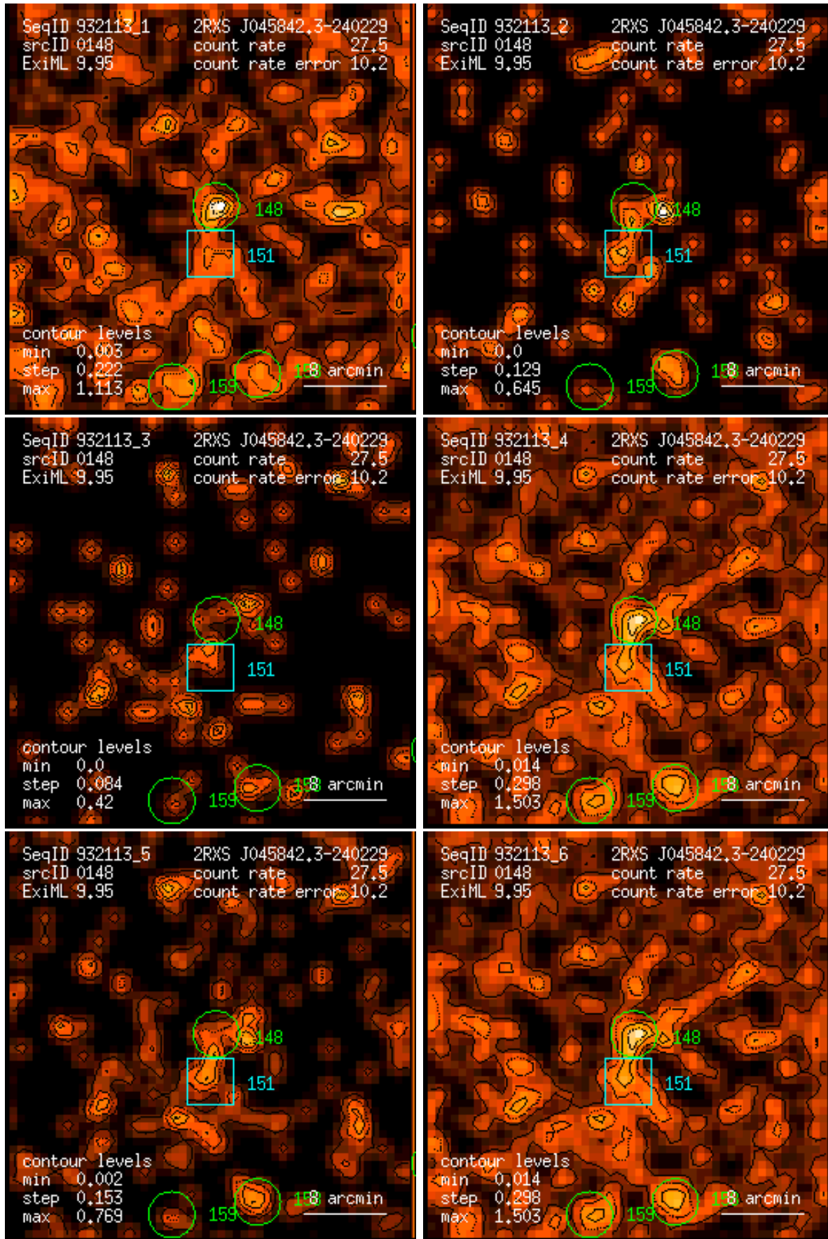
Figure 148: RASS 932113: detection 0148: band rate images, Gaussian filter: (1) PSPC channels 11 – 41, (2) 52 – 90, (3) 91 – 201, (4) 11 – 235, (5) 52 – 201, (6) 11 – 201. Broad band rates in counts/ks. Band rate contour levels in counts/ks/arcmin 2 .
