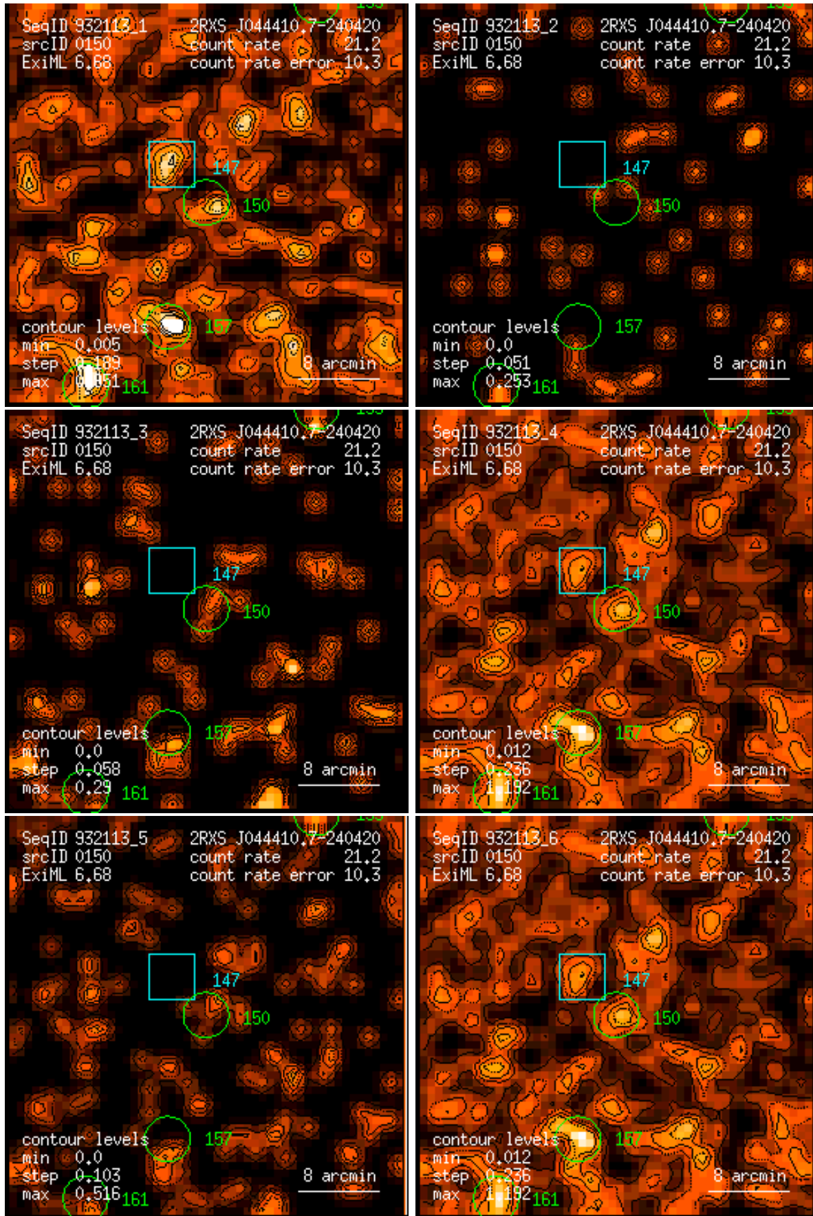
Figure 150: RASS 932113: detection 0150: band rate images, Gaussian filter: (1) PSPC channels 11 – 41, (2) 52 – 90, (3) 91 – 201, (4) 11 – 235, (5) 52 – 201, (6) 11 – 201. Broad band rates in counts/ks. Band rate contour levels in counts/ks/arcmin 2 .
