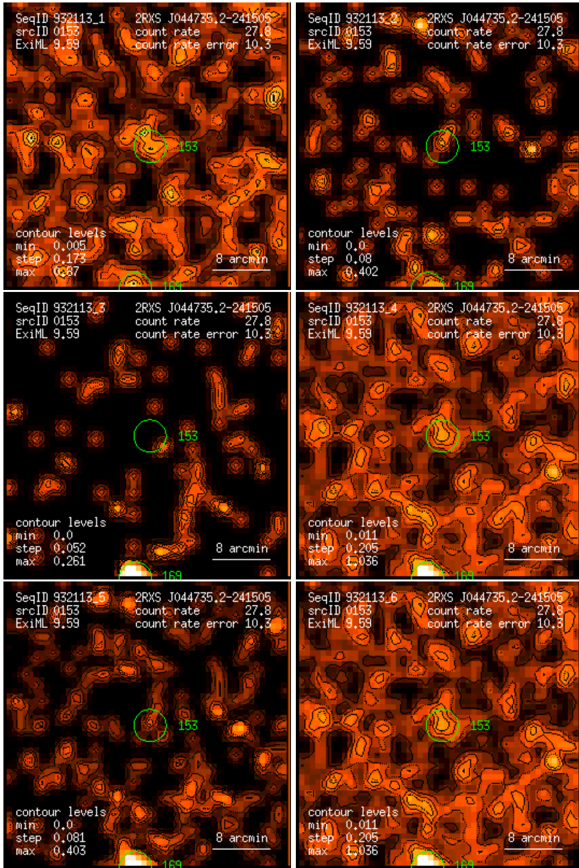
Figure 153: RASS 932113: detection 0153: band rate images, Gaussian filter: (1) PSPC channels 11 – 41, (2) 52 – 90, (3) 91 – 201, (4) 11 – 235, (5) 52 – 201, (6) 11 – 201. Broad band rates in counts/ks. Band rate contour levels in counts/ks/arcmin 2 .
