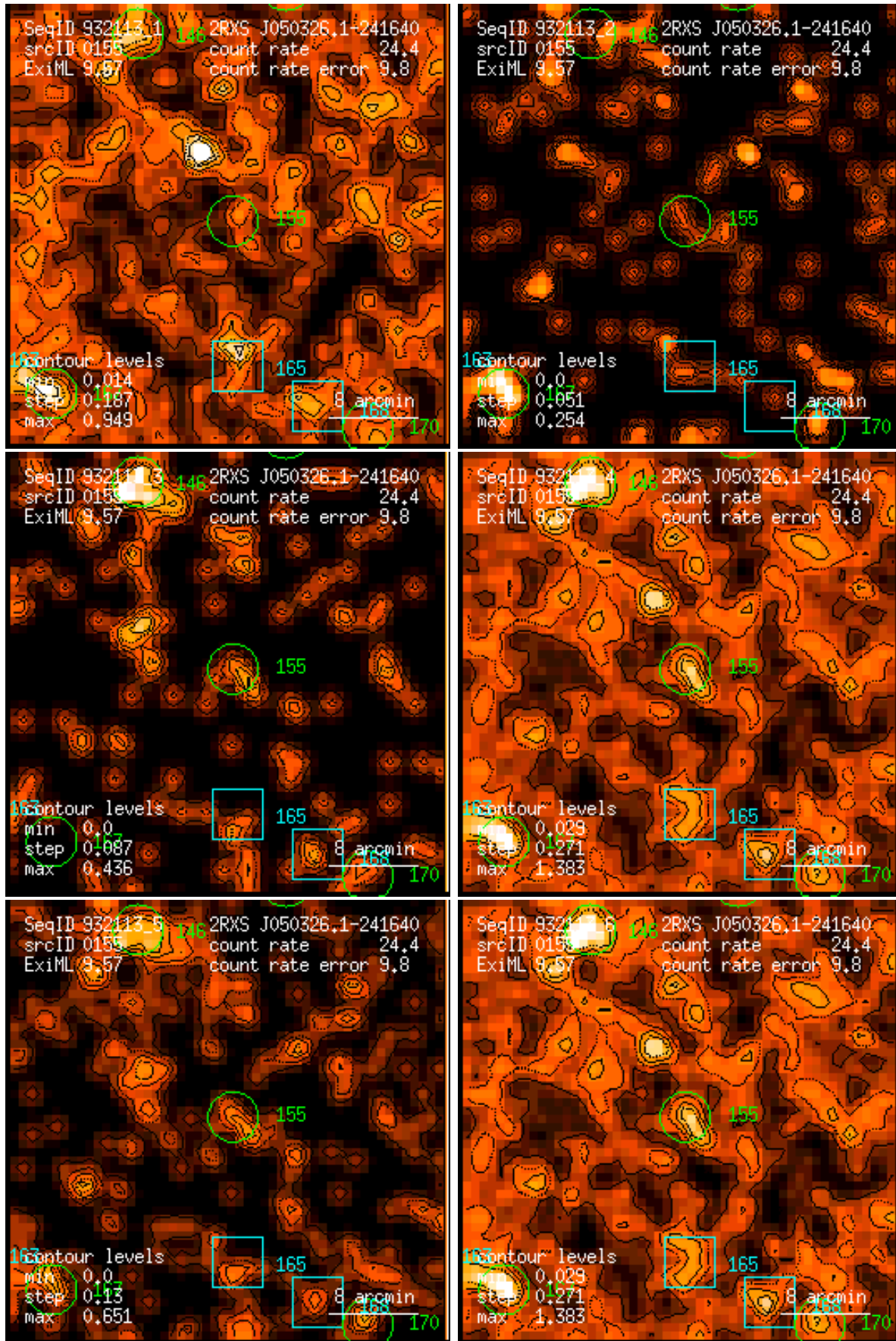
Figure 155: RASS 932113: detection 0155: band rate images, Gaussian filter: (1) PSPC channels 11 – 41, (2) 52 – 90, (3) 91 – 201, (4) 11 – 235, (5) 52 – 201, (6) 11 – 201. Broad band rates in counts/ks. Band rate contour levels in counts/ks/arcmin 2 .
