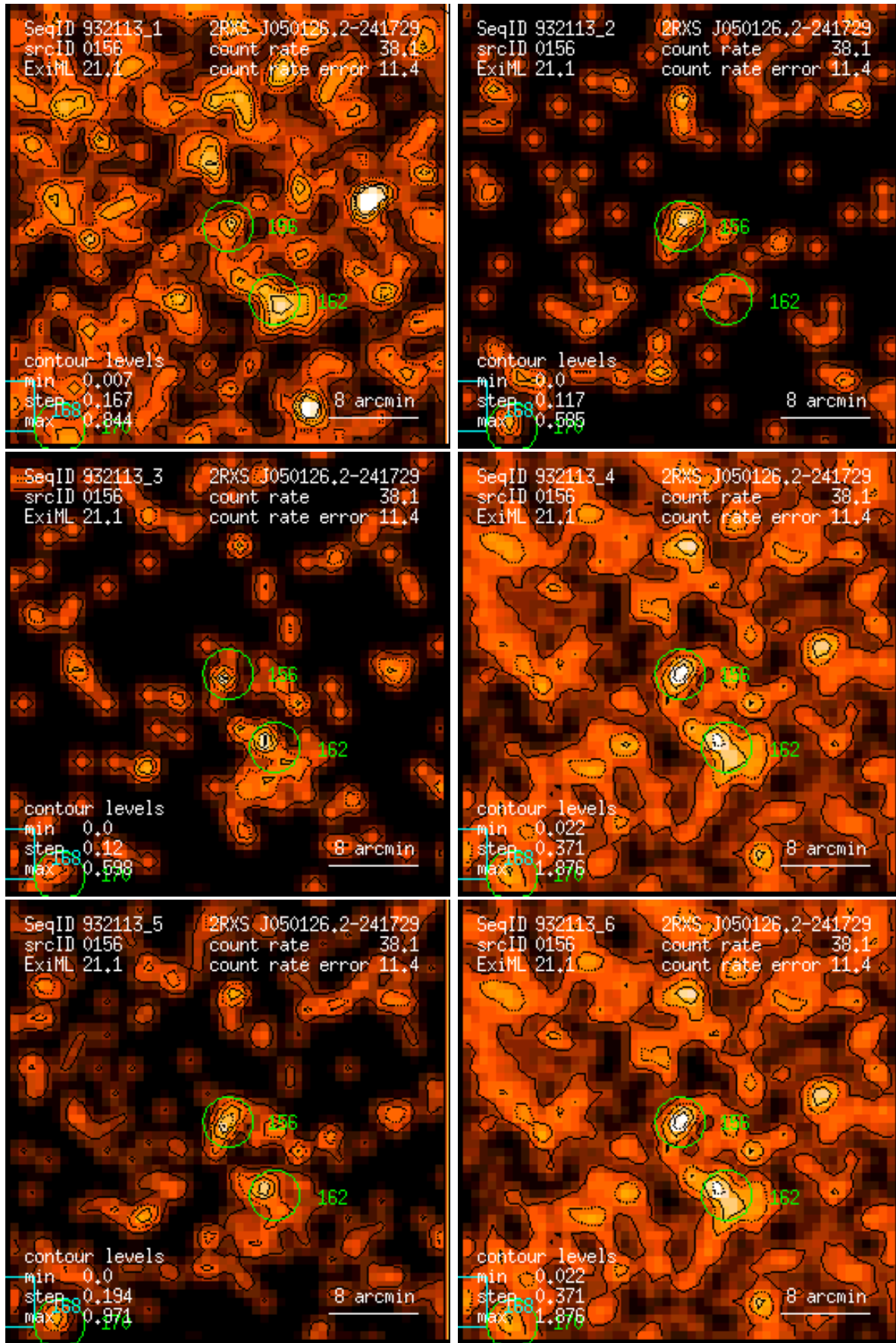
Figure 156: RASS 932113: detection 0156: band rate images, Gaussian filter: (1) PSPC channels 11 – 41, (2) 52 – 90, (3) 91 – 201, (4) 11 – 235, (5) 52 – 201, (6) 11 – 201. Broad band rates in counts/ks. Band rate contour levels in counts/ks/arcmin 2 .
