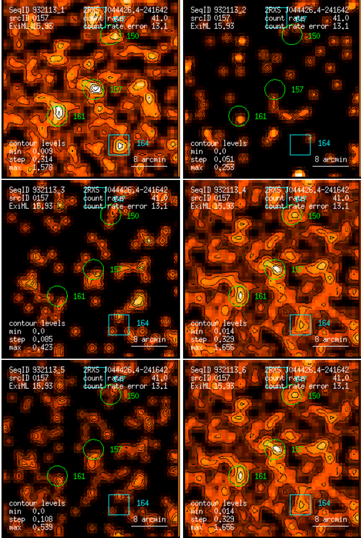
Figure 157: RASS 932113: detection 0157: band rate images, Gaussian filter: (1) PSPC channels 11 – 41, (2) 52 – 90, (3) 91 – 201, (4) 11 – 235, (5) 52 – 201, (6) 11 – 201. Broad band rates in counts/ks. Band rate contour levels in counts/ks/arcmin 2 .
