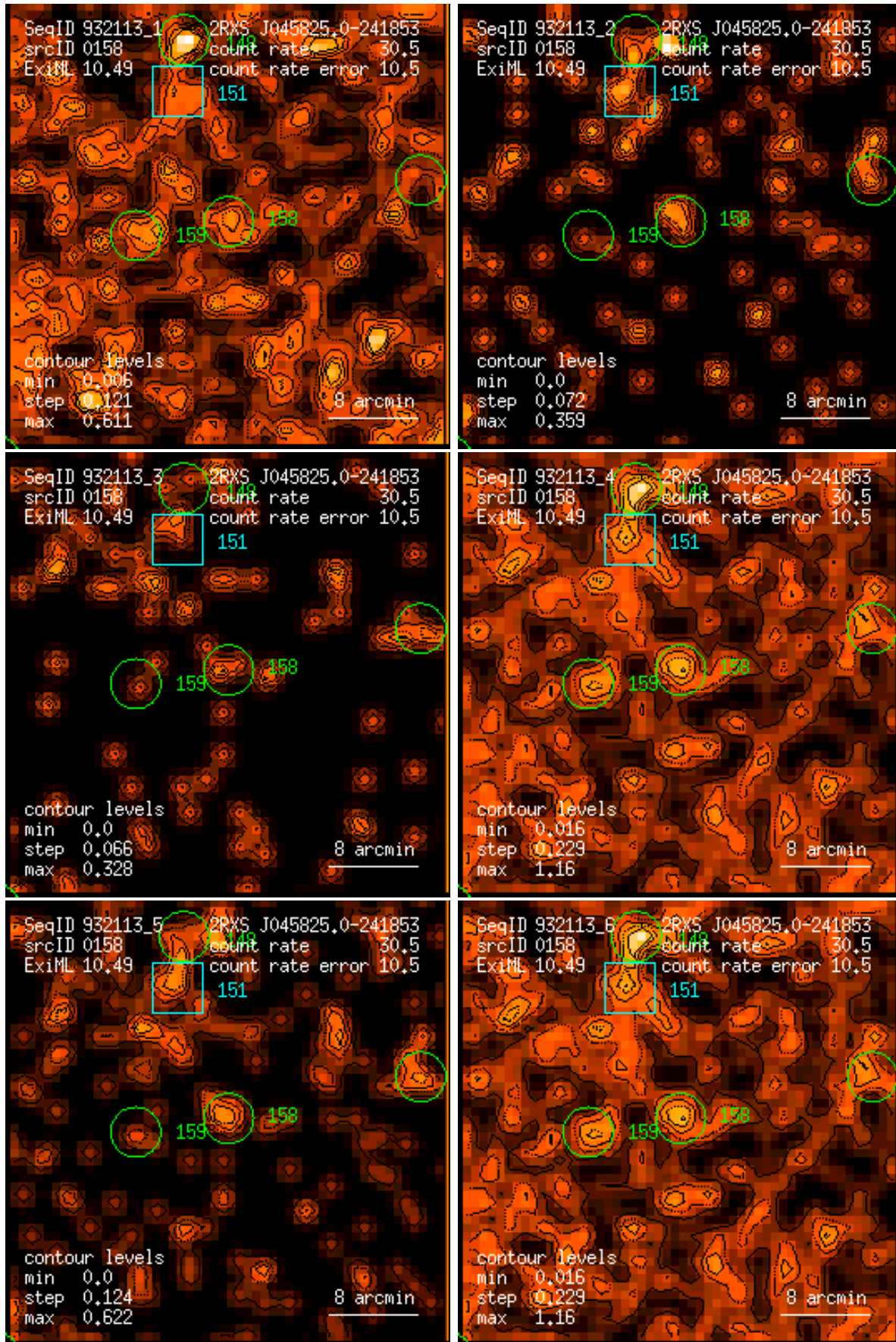
Figure 158: RASS 932113: detection 0158: band rate images, Gaussian filter: (1) PSPC channels 11 – 41, (2) 52 – 90, (3) 91 – 201, (4) 11 – 235, (5) 52 – 201, (6) 11 – 201. Broad band rates in counts/ks. Band rate contour levels in counts/ks/arcmin 2 .
