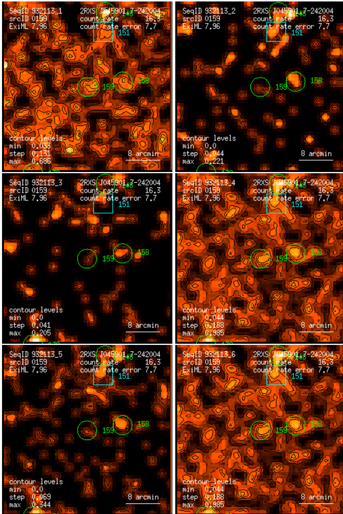
Figure 159: RASS 932113: detection 0159: band rate images, Gaussian filter: (1) PSPC channels 11 – 41, (2) 52 – 90, (3) 91 – 201, (4) 11 – 235, (5) 52 – 201, (6) 11 – 201. Broad band rates in counts/ks. Band rate contour levels in counts/ks/arcmin 2 .
