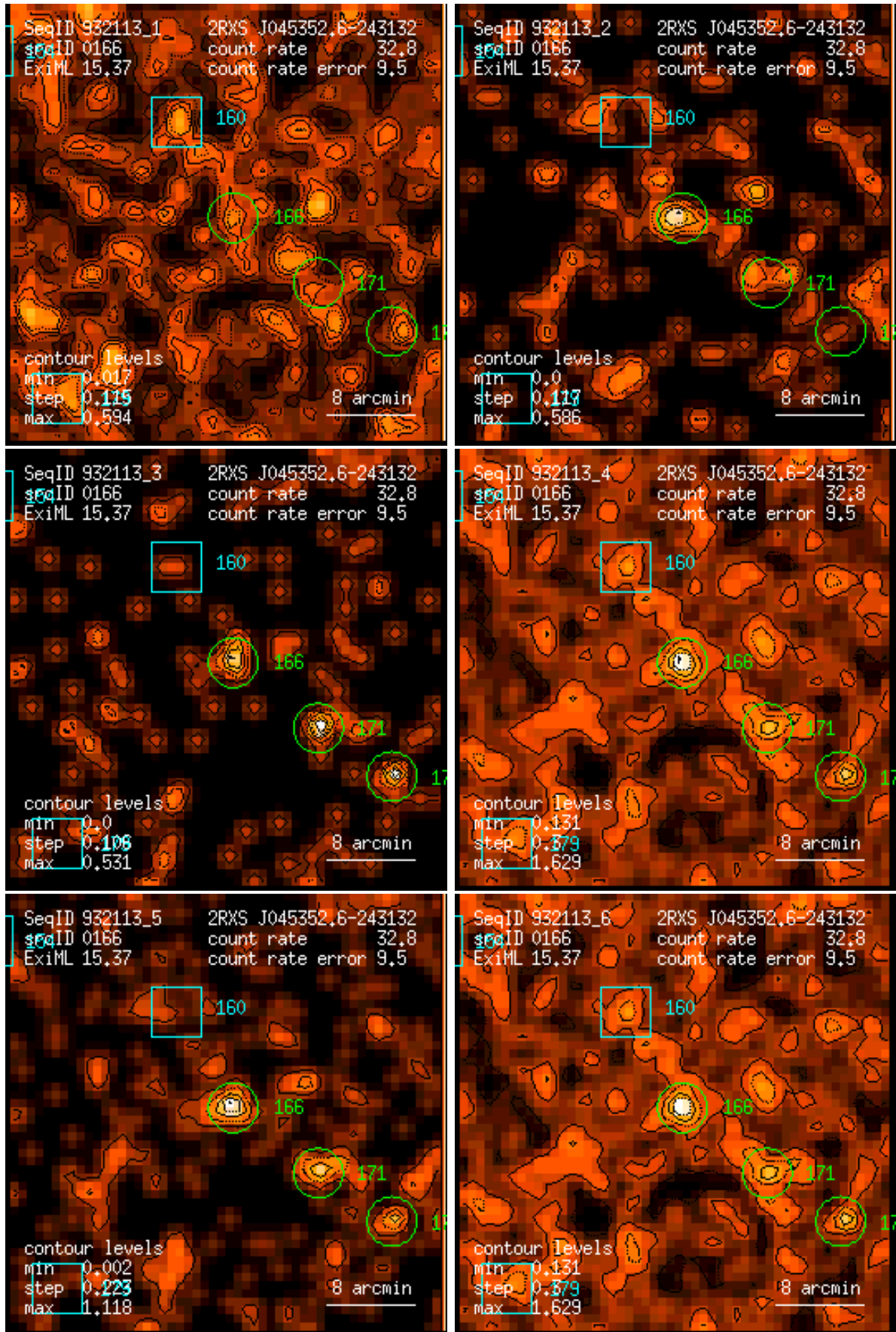
Figure 166: RASS 932113: detection 0166: band rate images, Gaussian filter: (1) PSPC channels 11 – 41, (2) 52 – 90, (3) 91 – 201, (4) 11 – 235, (5) 52 – 201, (6) 11 – 201. Broad band rates in counts/ks. Band rate contour levels in counts/ks/arcmin 2 .
