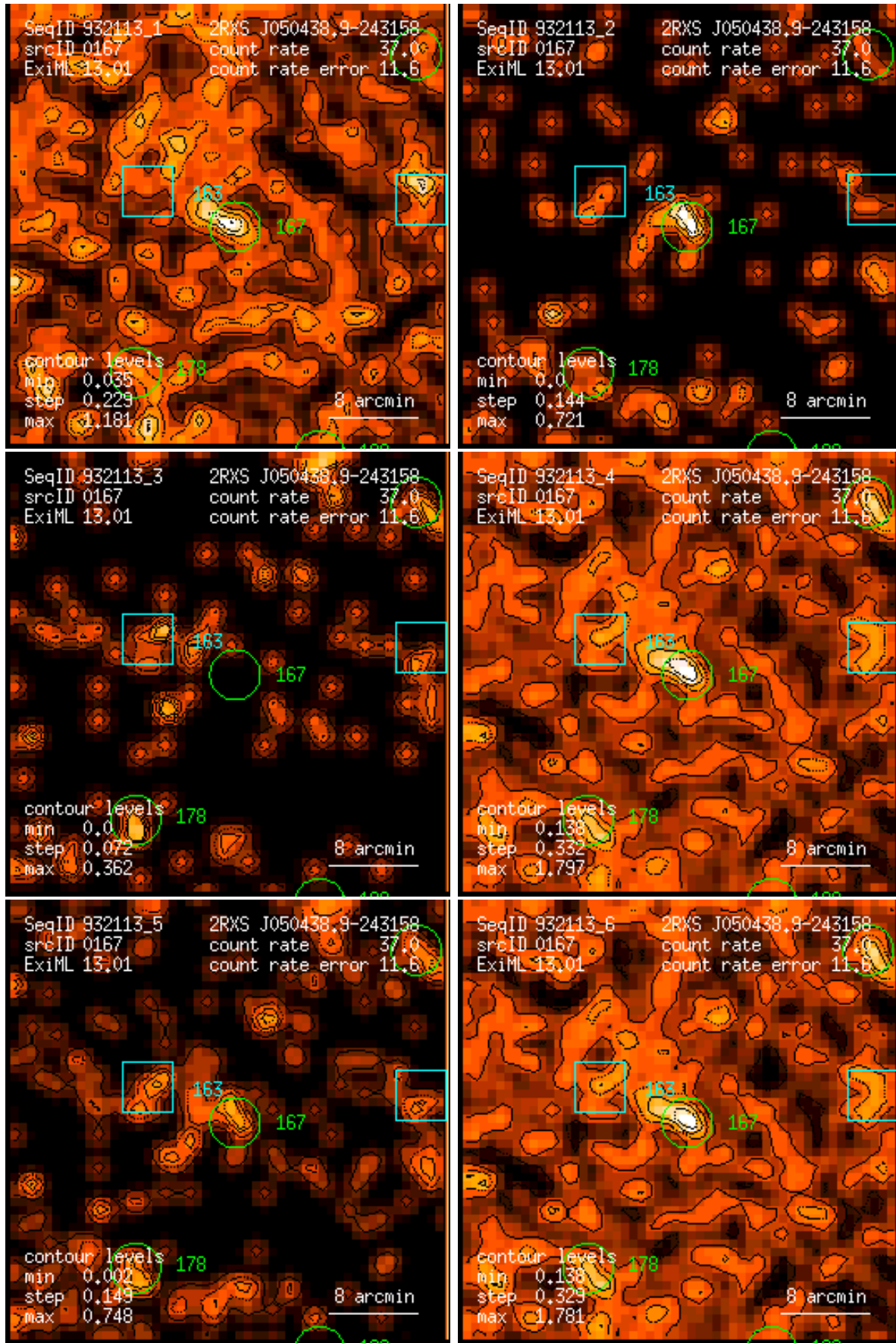
Figure 167: RASS 932113: detection 0167: band rate images, Gaussian filter: (1) PSPC channels 11 – 41, (2) 52 – 90, (3) 91 – 201, (4) 11 – 235, (5) 52 – 201, (6) 11 – 201. Broad band rates in counts/ks. Band rate contour levels in counts/ks/arcmin 2 .
